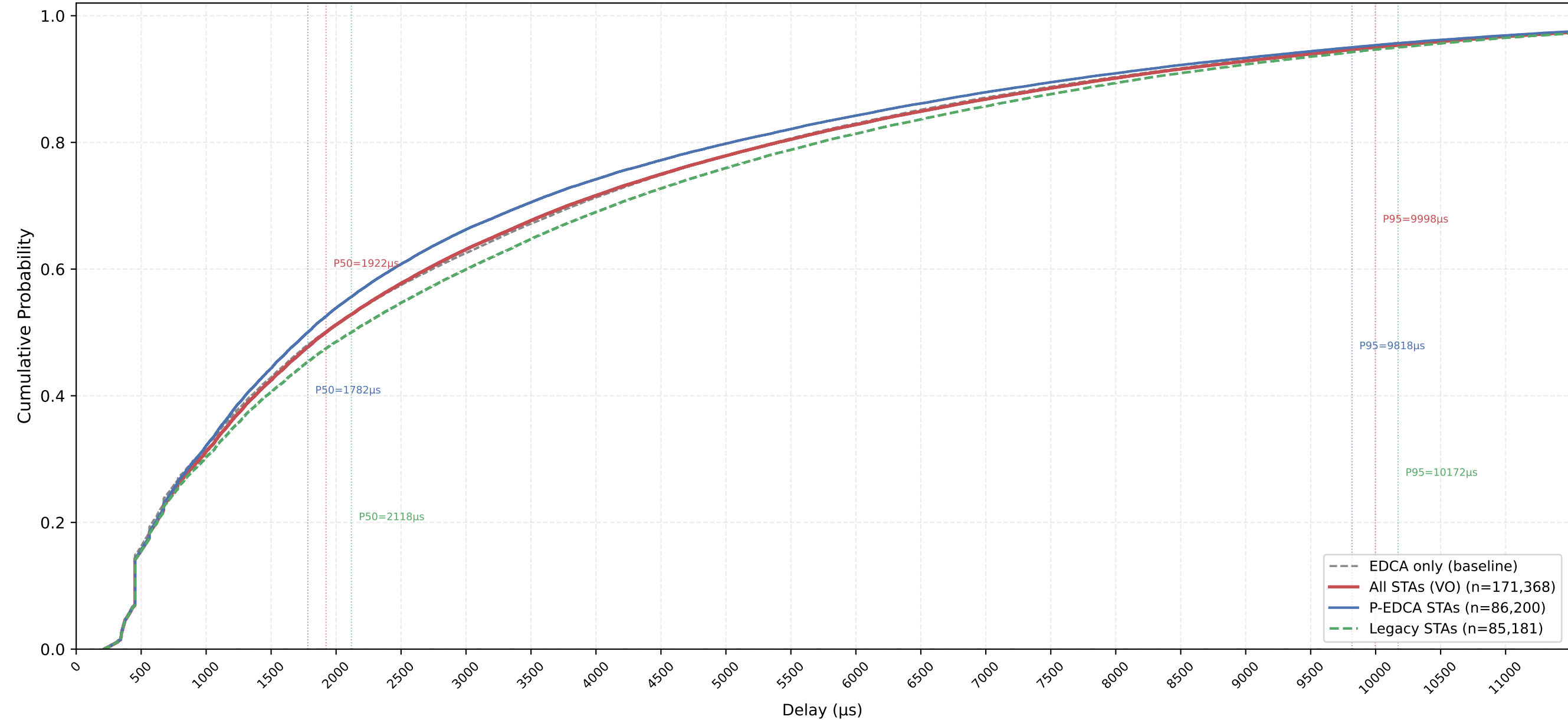
VO Delay CDF — P-EDCA / Legacy / All | CWds=0 × QSRC=1 × PSRC=2 nSta=30, nPedca=15/30, 1Mbps, avg of 10 runs
