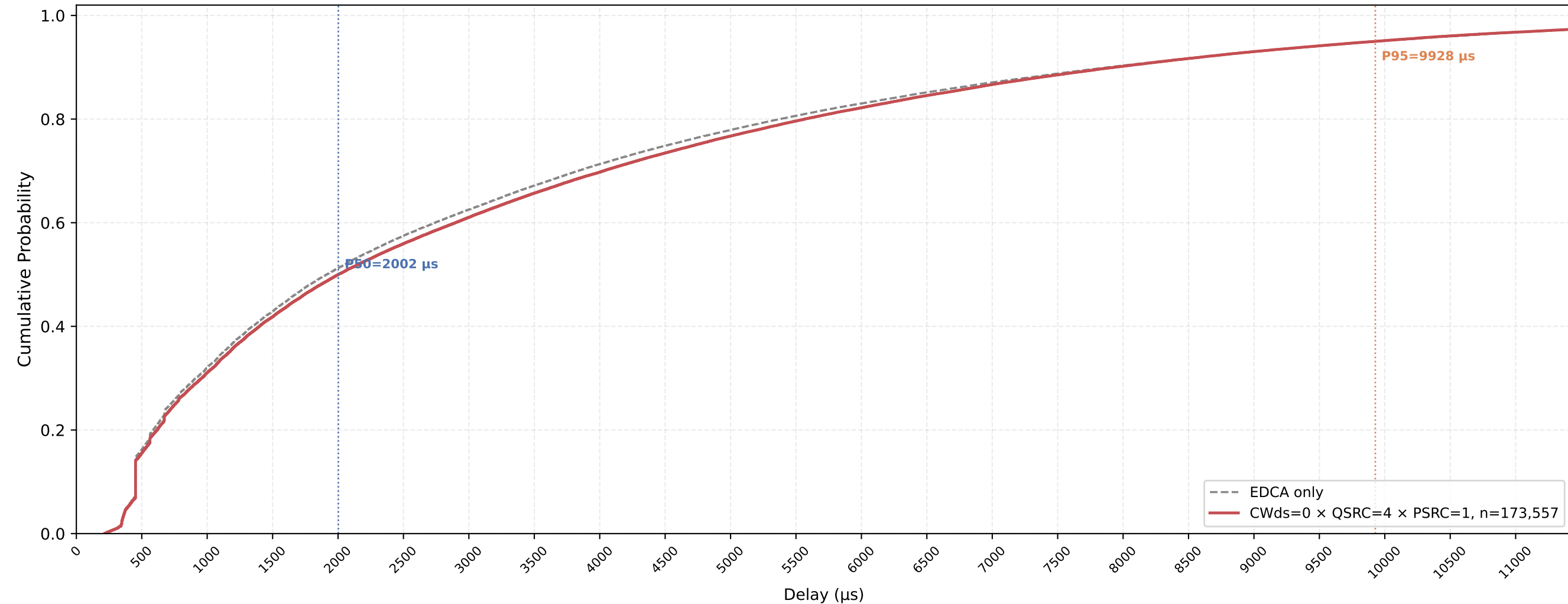
VO (all STAs) Delay CDF — CWds=0 × QSRC=4 × PSRC=1 nSta=30, nPedca=30, 1Mbps, avg of 10 runs
