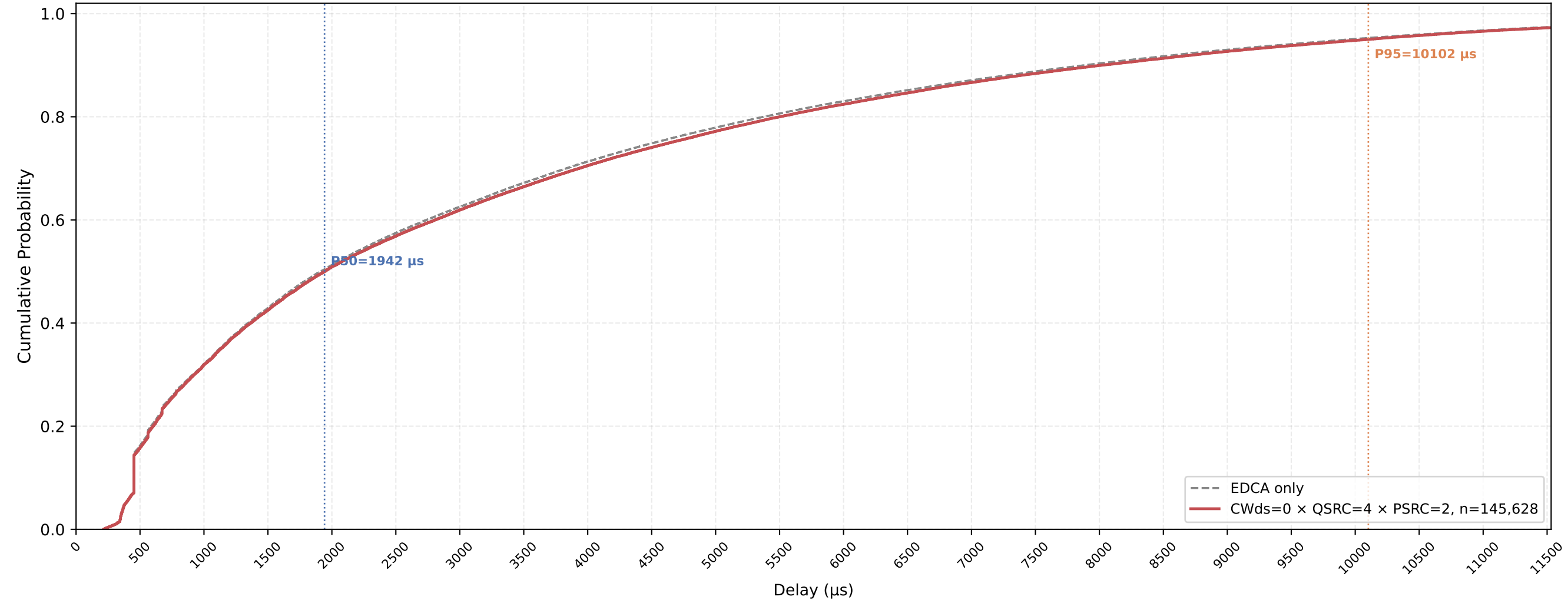
Legacy STA VO Delay CDF — CWds=0 × QSRC=4 × PSRC=2 nSta=30, nPedca=5, 1Mbps, avg of 10 runs
