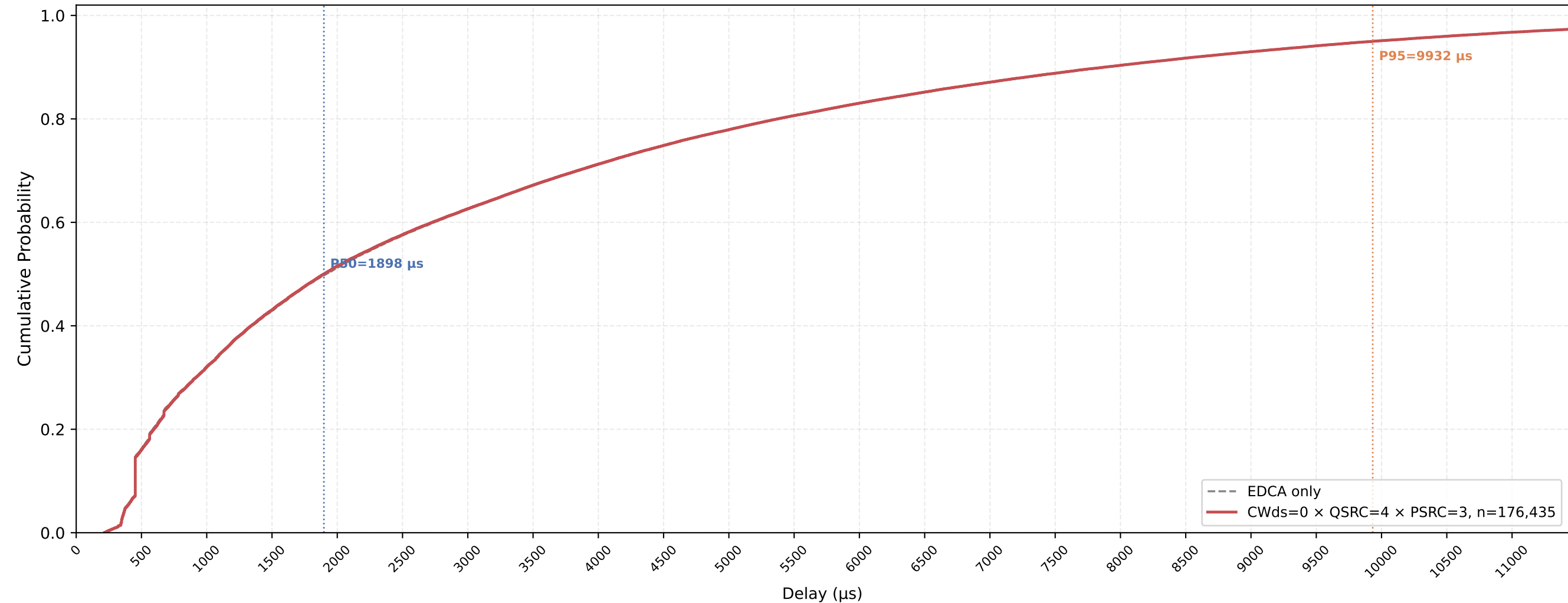
VO (all STAs) Delay CDF — CWds=0 × QSRC=4 × PSRC=3 nSta=30, nPedca=5, 1Mbps, avg of 10 runs
