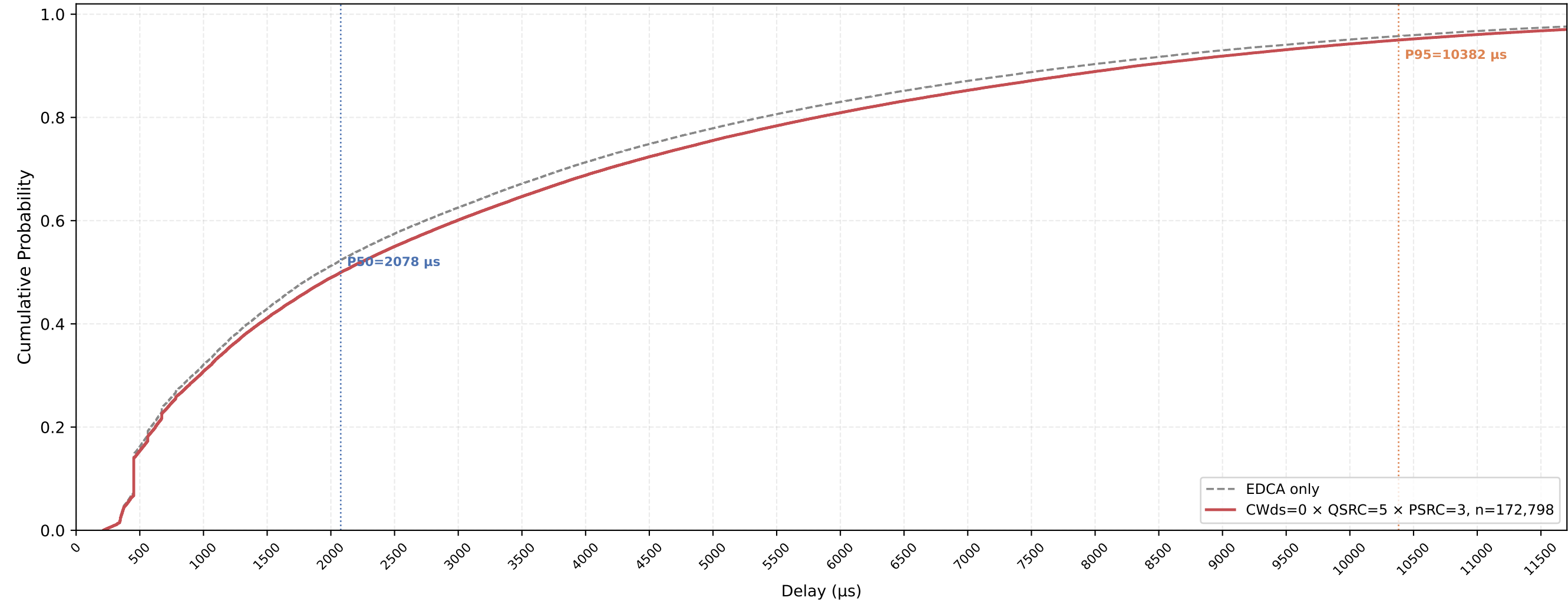
P-EDCA STA VO Delay CDF — CWds=0 × QSRC=5 × PSRC=3 nSta=30, nPedca=30, 1Mbps, avg of 10 runs
