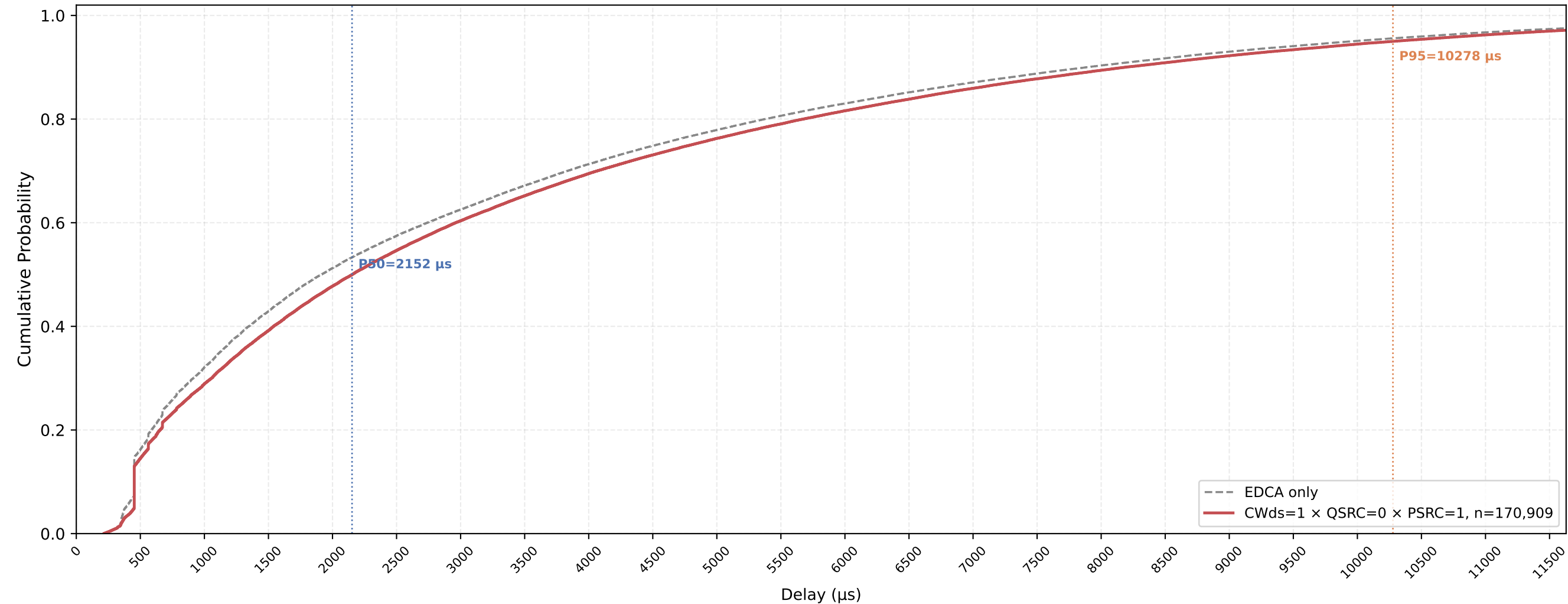
VO (all STAs) Delay CDF — CWds=1 × QSRC=0 × PSRC=1 nSta=30, nPedca=15, 1Mbps, avg of 10 runs
