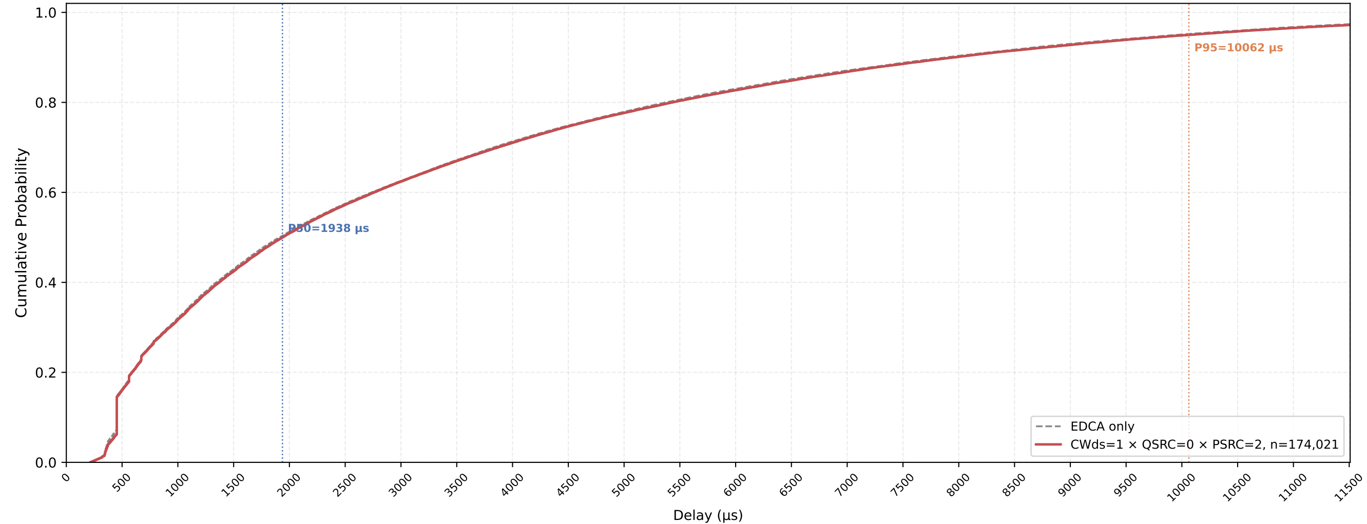
VO (all STAs) Delay CDF — CWds=1 × QSRC=0 × PSRC=2 nSta=30, nPedca=5, 1Mbps, avg of 10 runs
