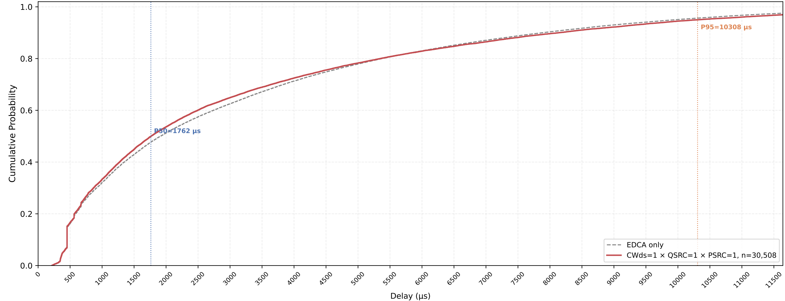
P-EDCA STA VO Delay CDF — CWds=1 × QSRC=1 × PSRC=1 nSta=30, nPedca=5, 1Mbps, avg of 10 runs
