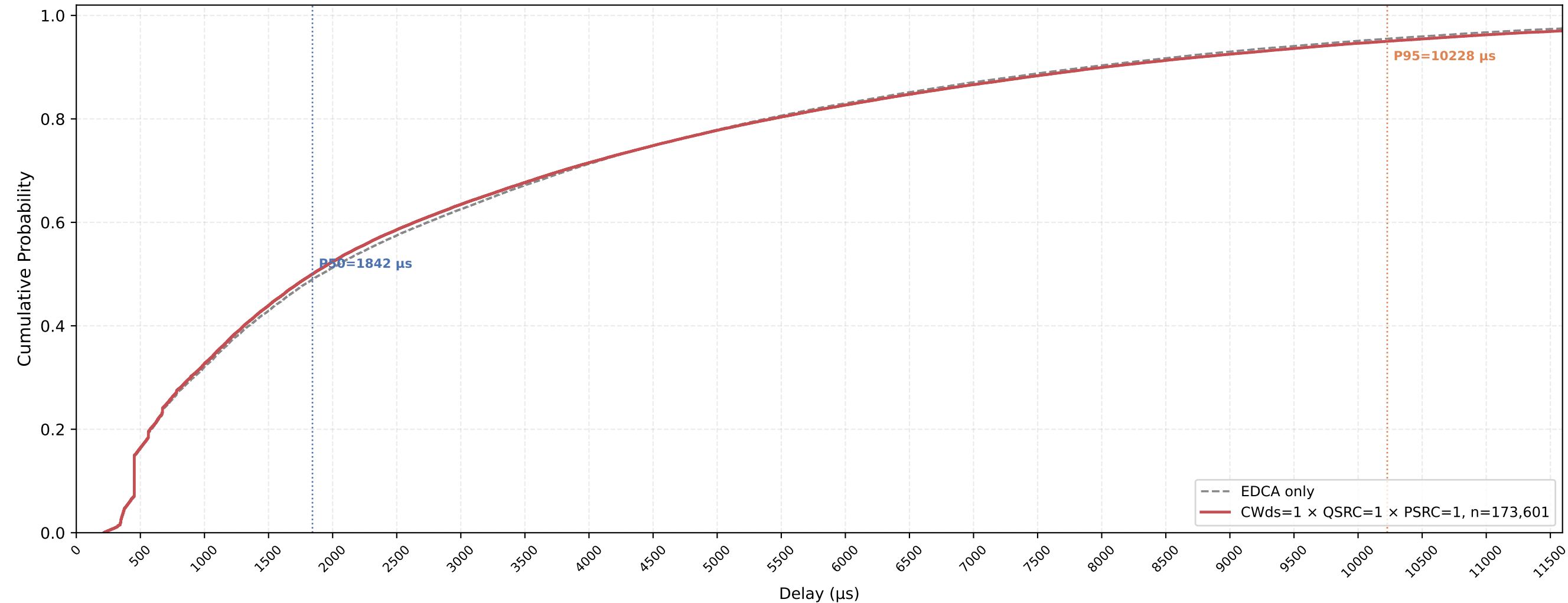
VO (all STAs) Delay CDF — CWds=1 × QSRC=1 × PSRC=1 nSta=30, nPedca=15, 1Mbps, avg of 10 runs
