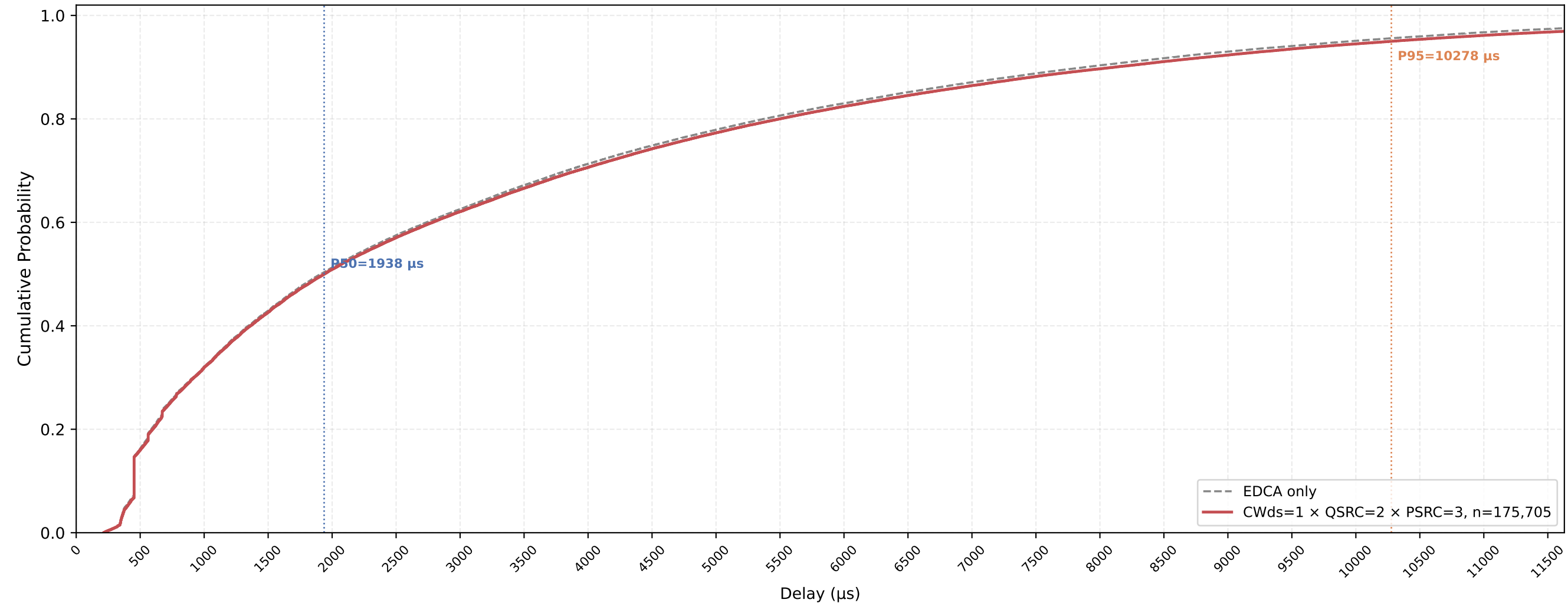
VO (all STAs) Delay CDF — CWds=1 × QSRC=2 × PSRC=3 nSta=30, nPedca=5, 1Mbps, avg of 10 runs
