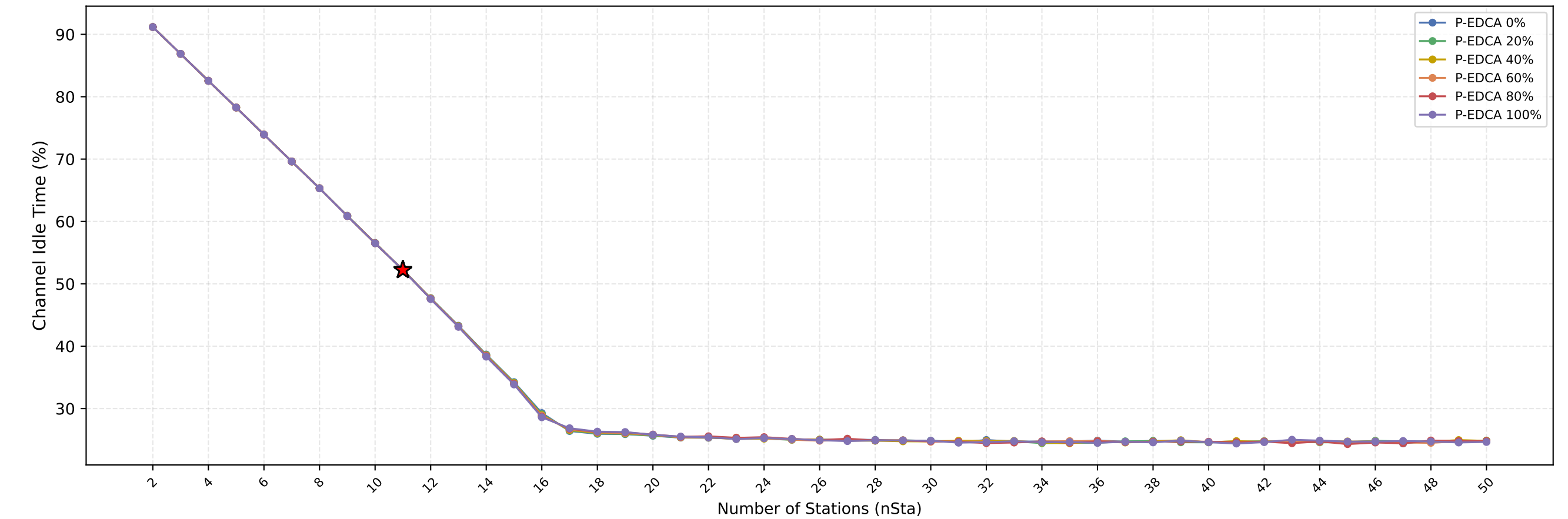
Channel Idle Time vs nSta — (Red Star = Current nSta=11)
