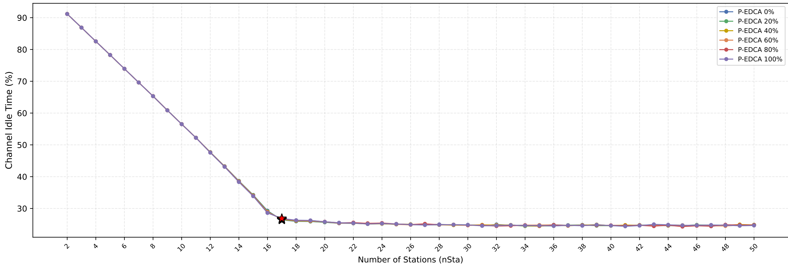
Channel Idle Time vs nSta — (Red Star = Current nSta=17)
