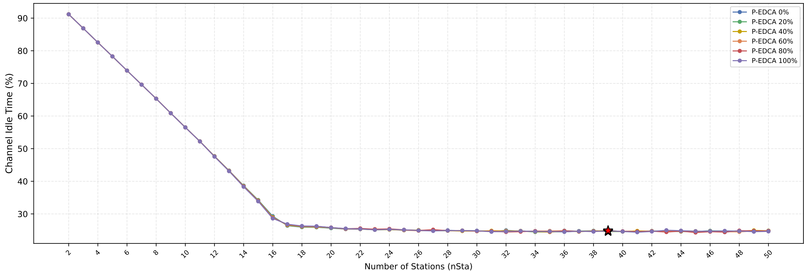
Channel Idle Time vs nSta — (Red Star = Current nSta=39)
