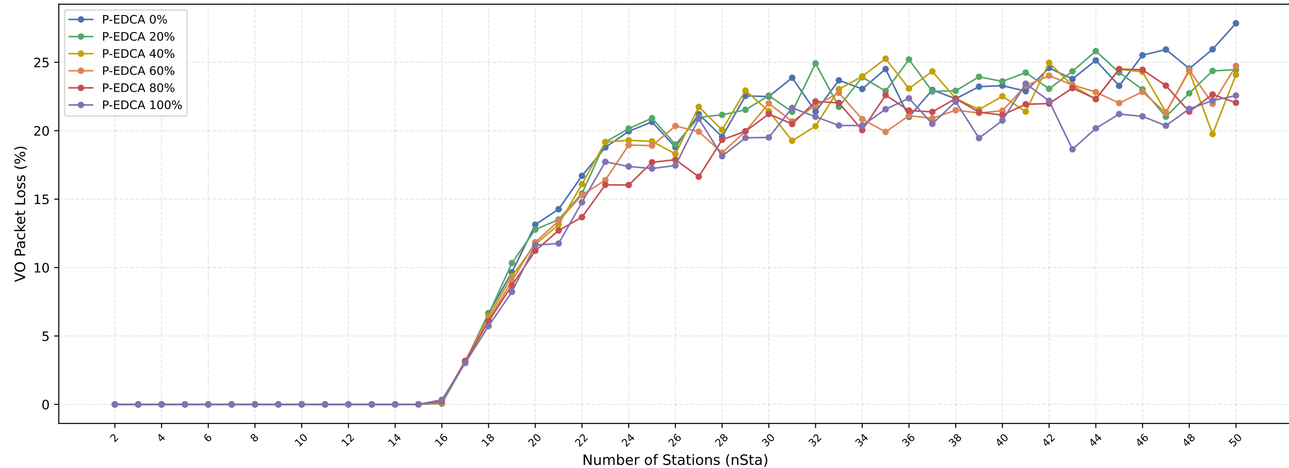
VO Packet Loss vs nSta — 1Mbps (avg of 10 runs)
