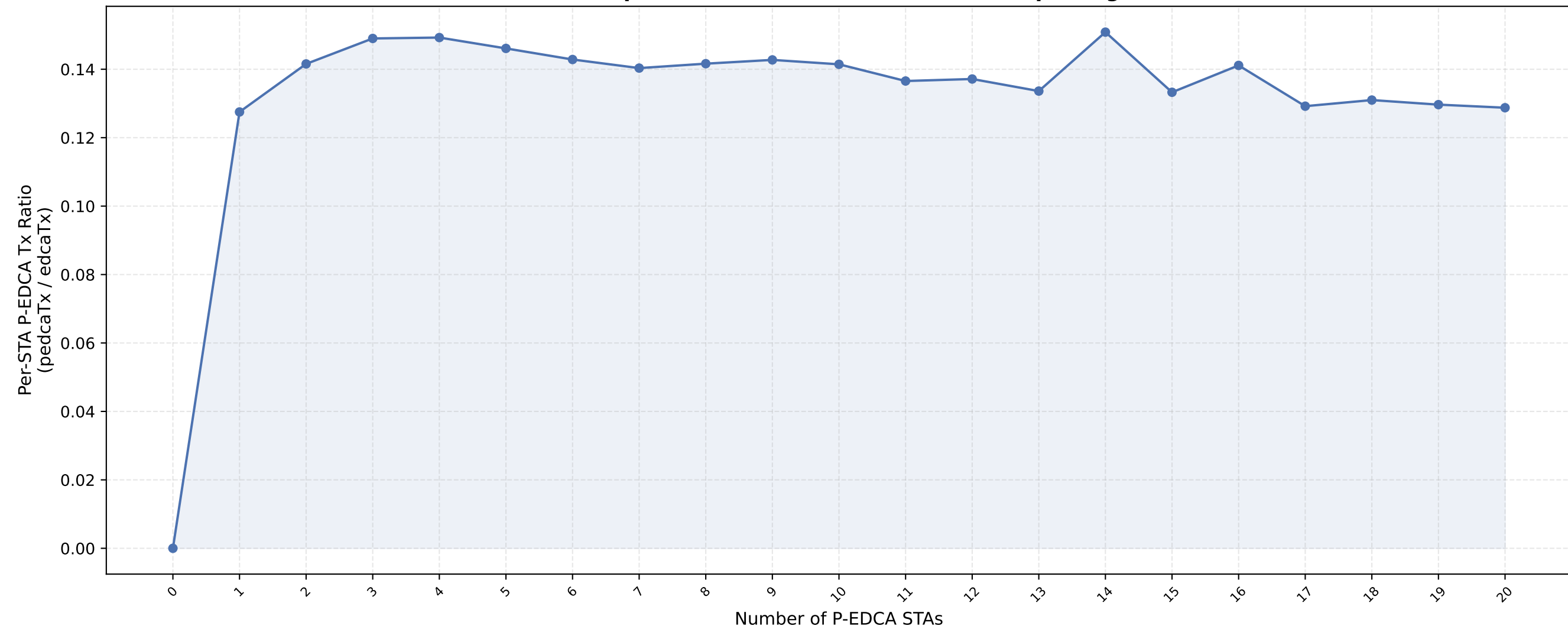
Per-P-EDCA-STA: pedcaTx / edcaTx — nSta=20, 1Mbps (avg of 10 runs)
