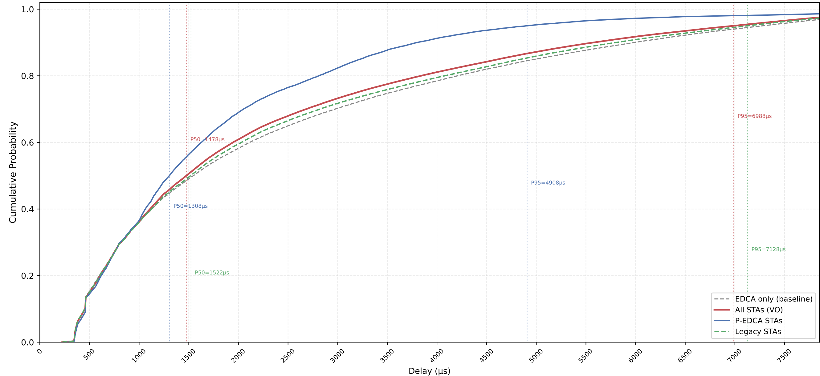
VO Delay CDF — P-EDCA / Legacy / All | CWds=0 × QSRC=1 × PSRC=1 nSta=30, nPedca=5/30, 1Mbps, avg of 10 runs
