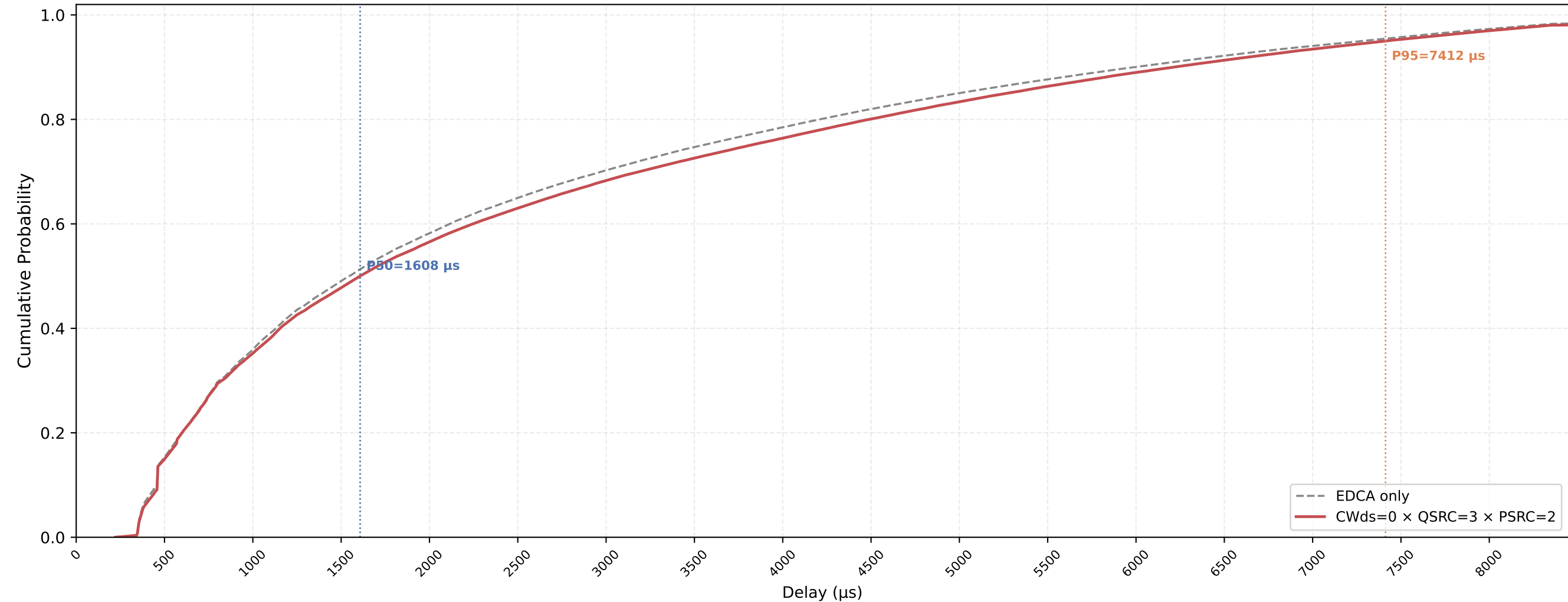
VO (all STAs) Delay CDF — CWds=0 × QSRC=3 × PSRC=2 nSta=30, nPedca=15, 1Mbps, avg of 10 runs
