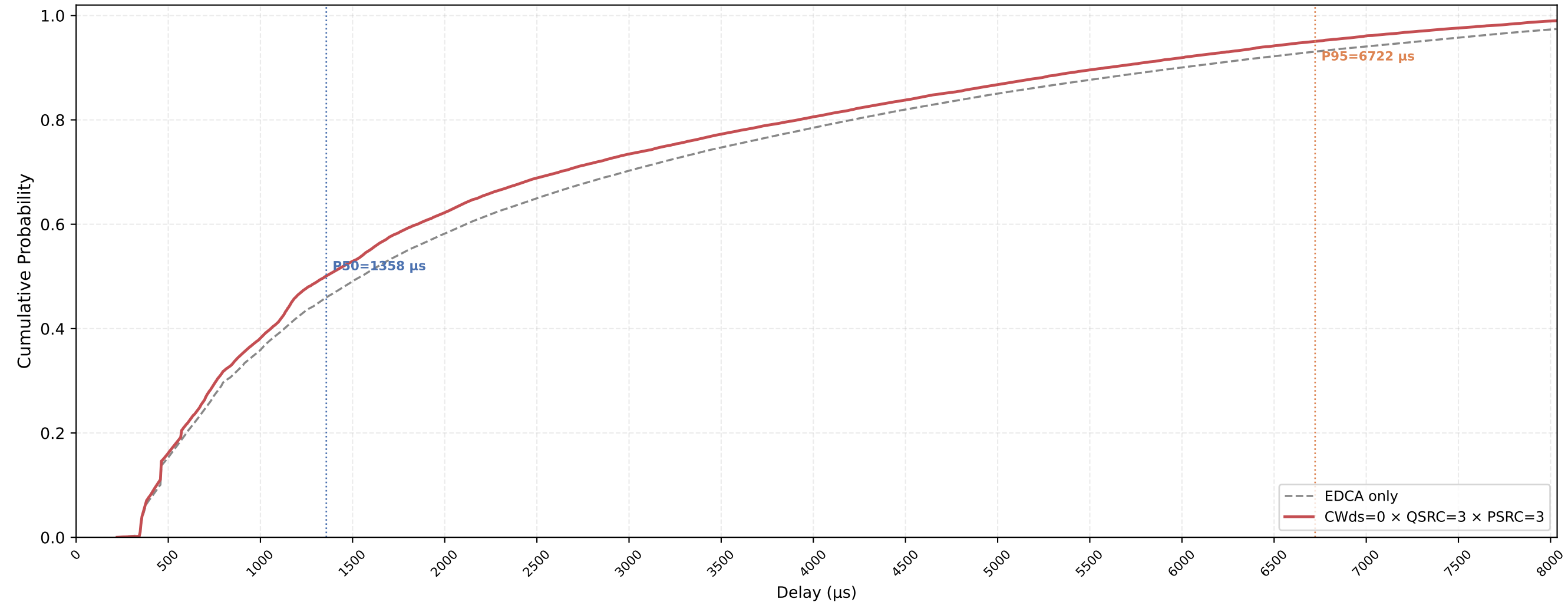
P-EDCA STA VO Delay CDF — CWds=0 × QSRC=3 × PSRC=3 nSta=30, nPedca=5, 1Mbps, avg of 10 runs
