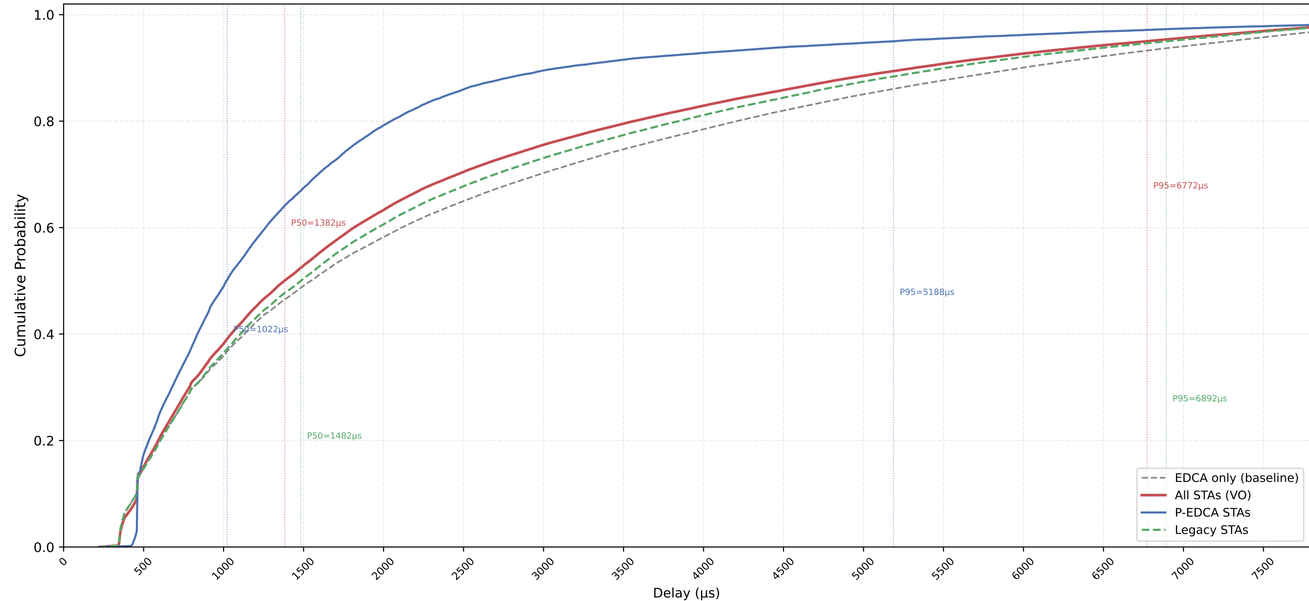
VO Delay CDF — P-EDCA / Legacy / All | CWds=1 × QSRC=0 × PSRC=1 nSta=30, nPedca=5/30, 1Mbps, avg of 10 runs
