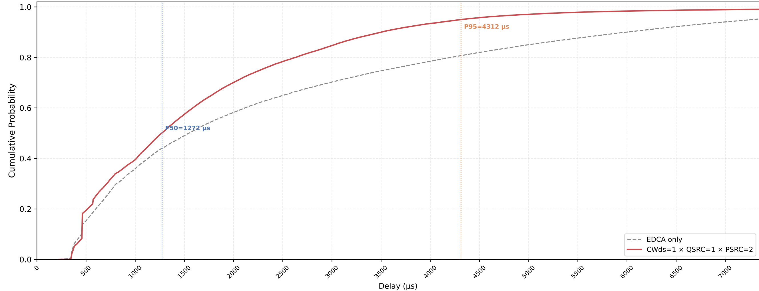
P-EDCA STA VO Delay CDF — CWds=1 × QSRC=1 × PSRC=2 nSta=30, nPedca=15, 1Mbps, avg of 10 runs
