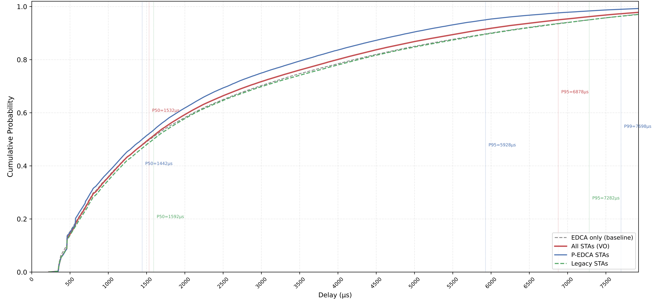
VO Delay CDF — P-EDCA / Legacy / All | CWds=1 × QSRC=2 × PSRC=3 nSta=30, nPedca=15/30, 1Mbps, avg of 10 runs
