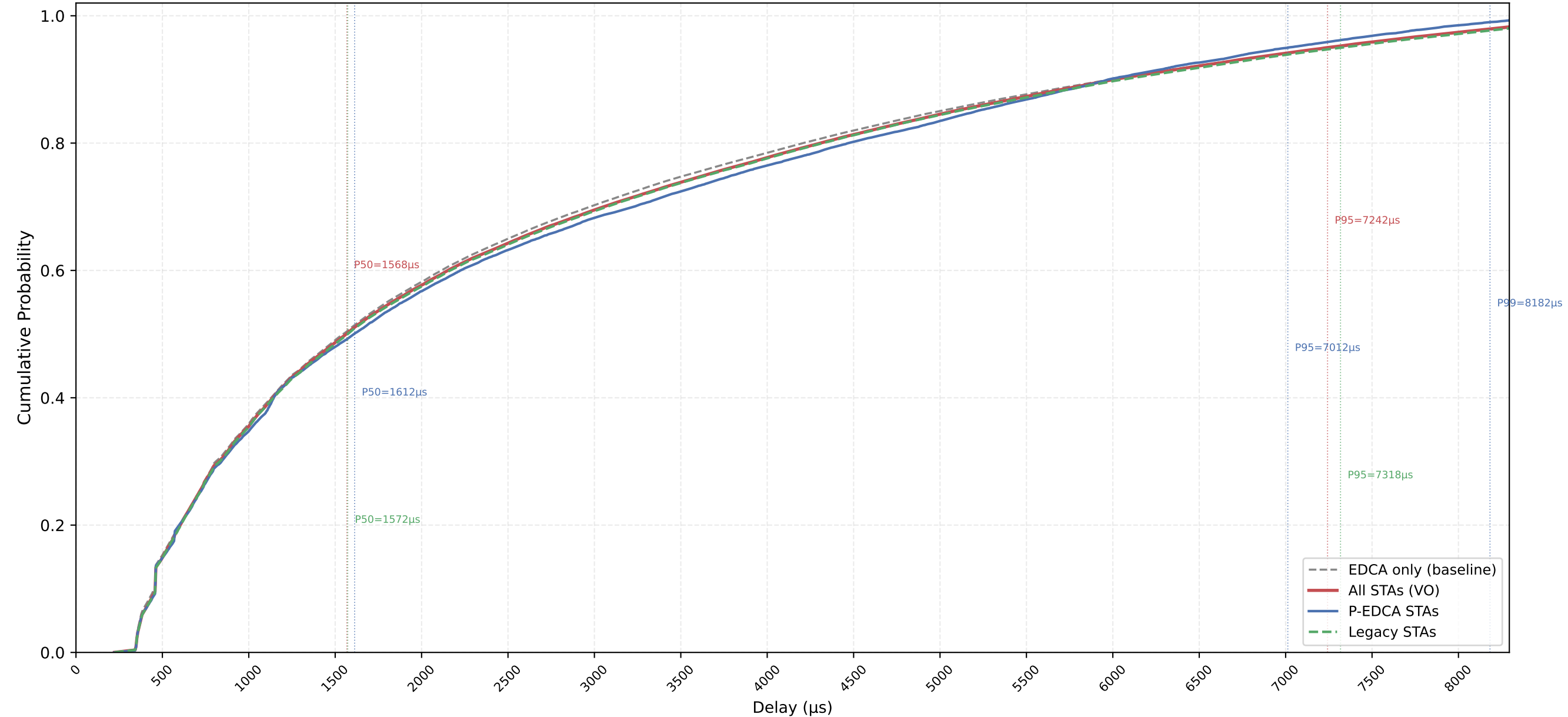
VO Delay CDF — P-EDCA / Legacy / All | CWds=1 × QSRC=3 × PSRC=2 nSta=30, nPedca=5/30, 1Mbps, avg of 10 runs
