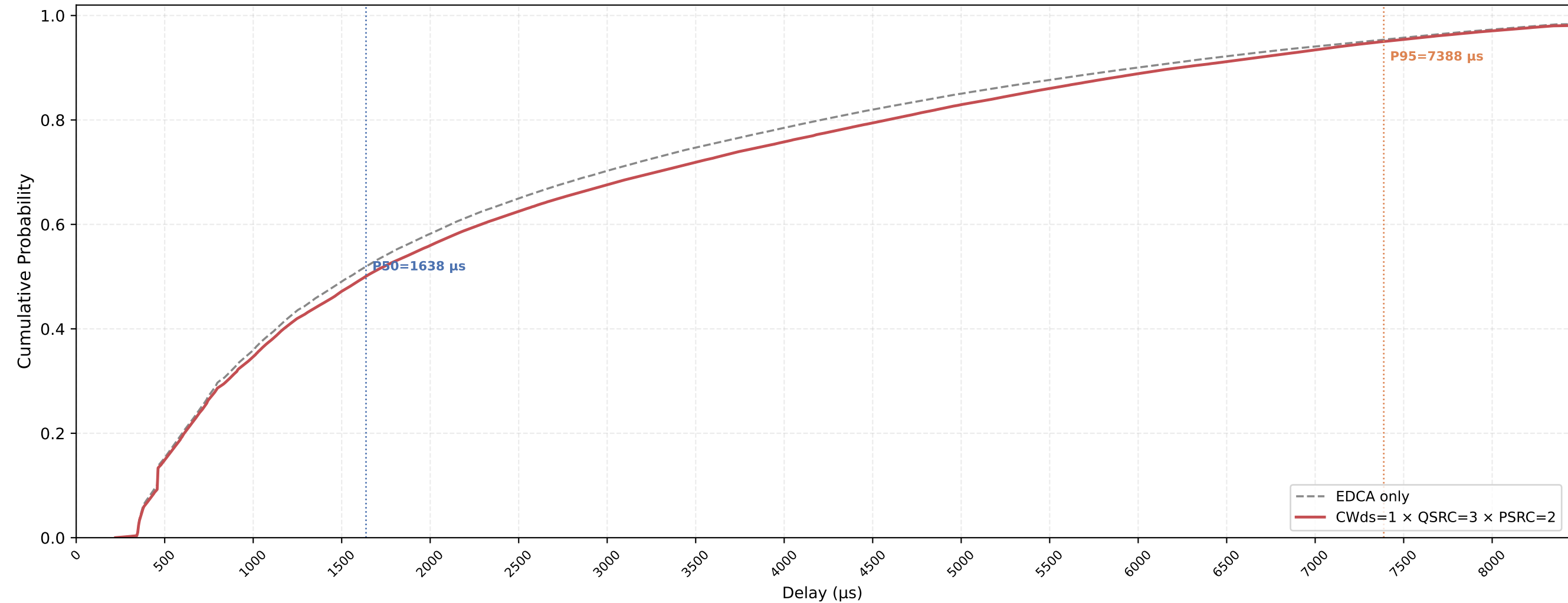
Legacy STA VO Delay CDF — CWds=1 × QSRC=3 × PSRC=2 nSta=30, nPedca=15, 1Mbps, avg of 10 runs
