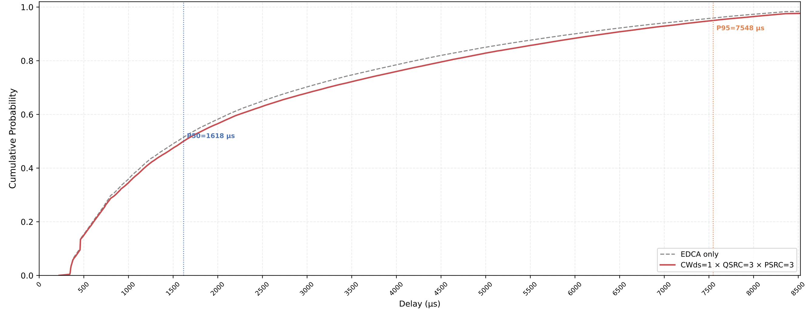
Legacy STA VO Delay CDF — CWds=1 × QSRC=3 × PSRC=3 nSta=30, nPedca=15, 1Mbps, avg of 10 runs
