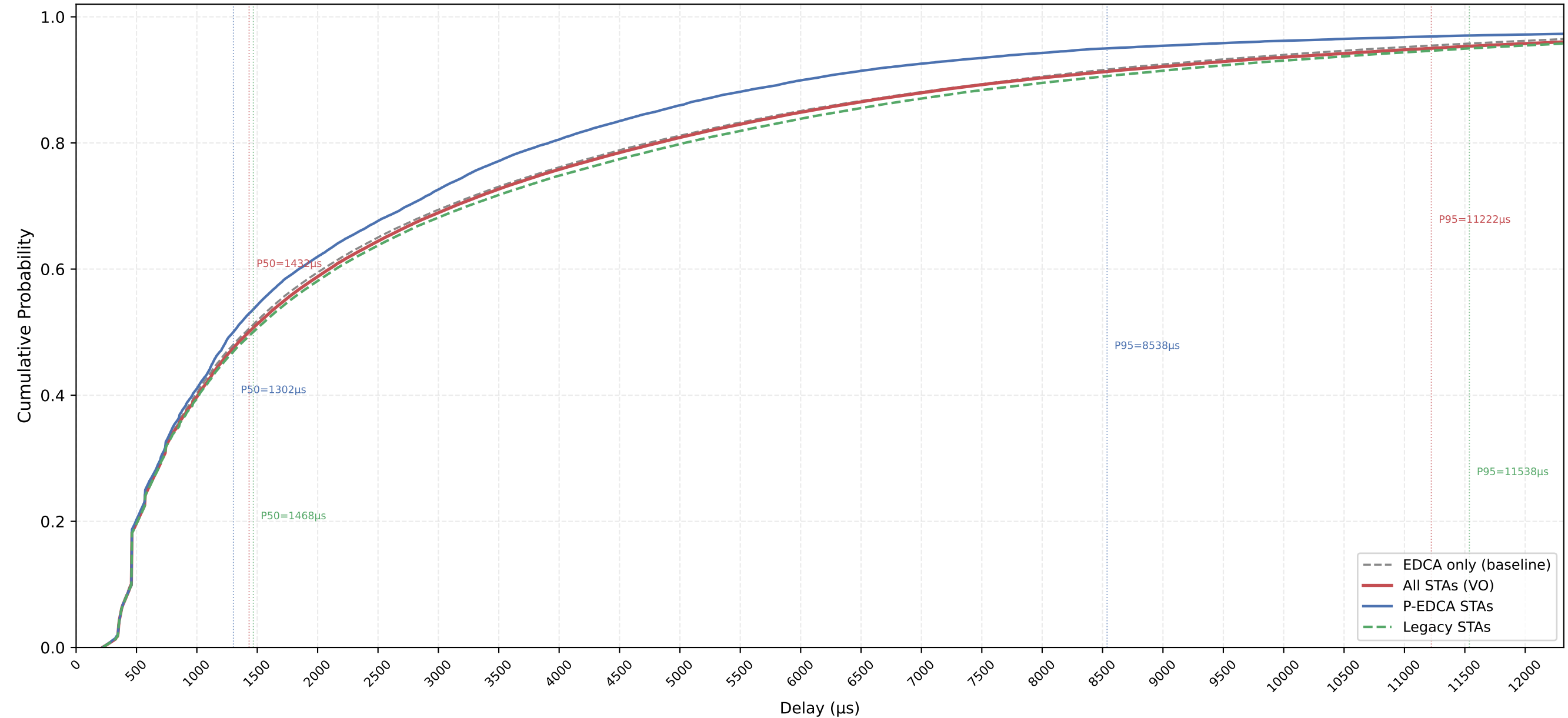
VO Delay CDF — P-EDCA / Legacy / All | CWds=0 × QSRC=2 × PSRC=1 nSta=30, nPedca=5/30, 1Mbps, avg of 10 runs
