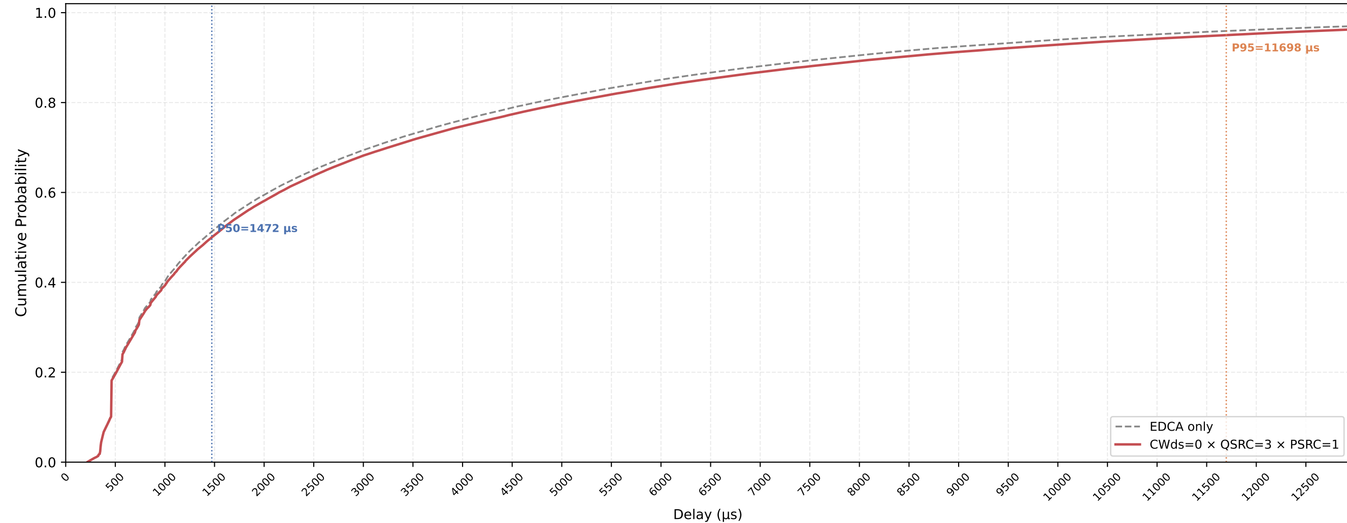
Legacy STA VO Delay CDF — CWds=0 × QSRC=3 × PSRC=1 nSta=30, nPedca=5, 1Mbps, avg of 10 runs
