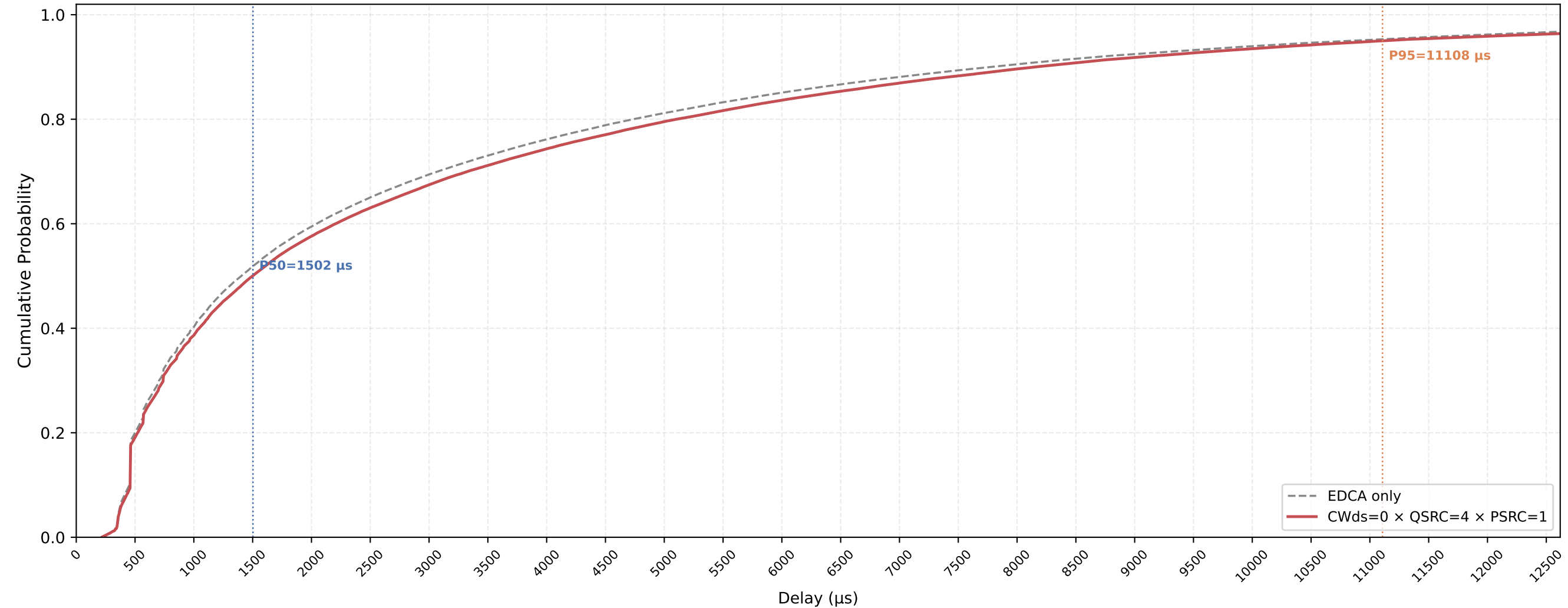
P-EDCA STA VO Delay CDF — CWds=0 × QSRC=4 × PSRC=1 nSta=30, nPedca=15, 1Mbps, avg of 10 runs
