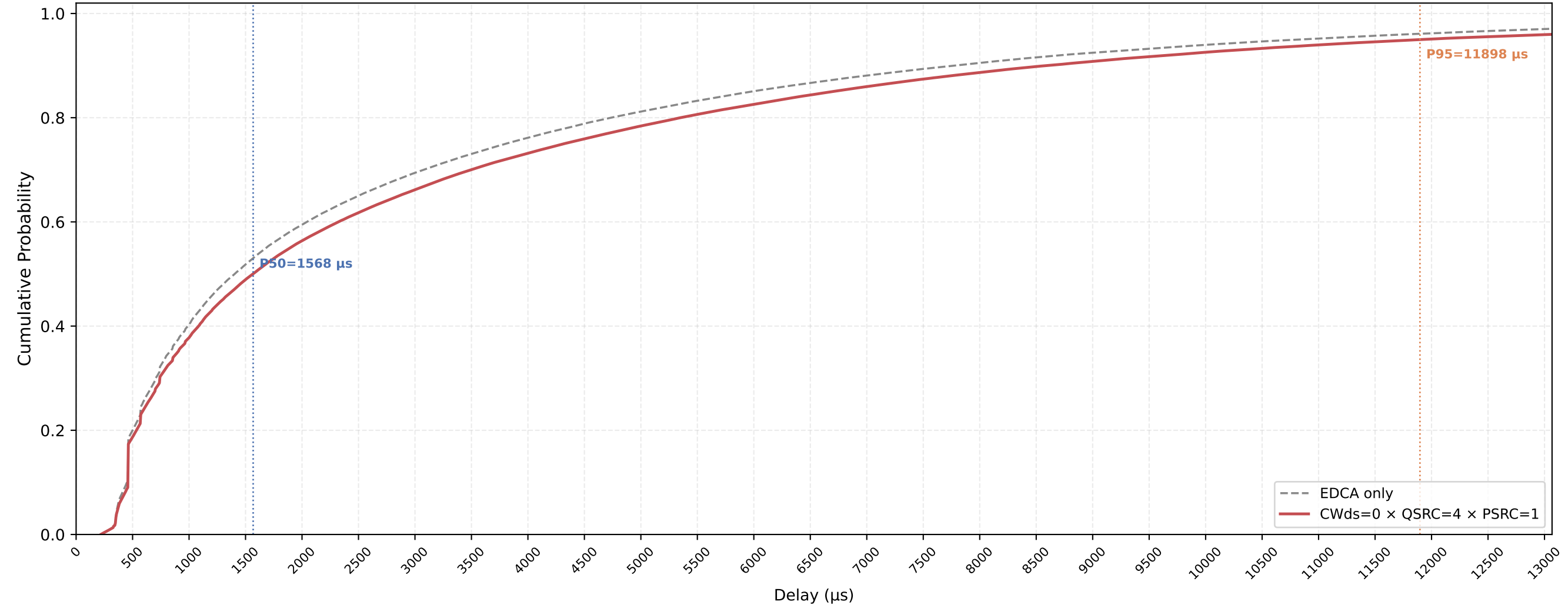
P-EDCA STA VO Delay CDF — CWds=0 × QSRC=4 × PSRC=1 nSta=30, nPedca=30, 1Mbps, avg of 10 runs
