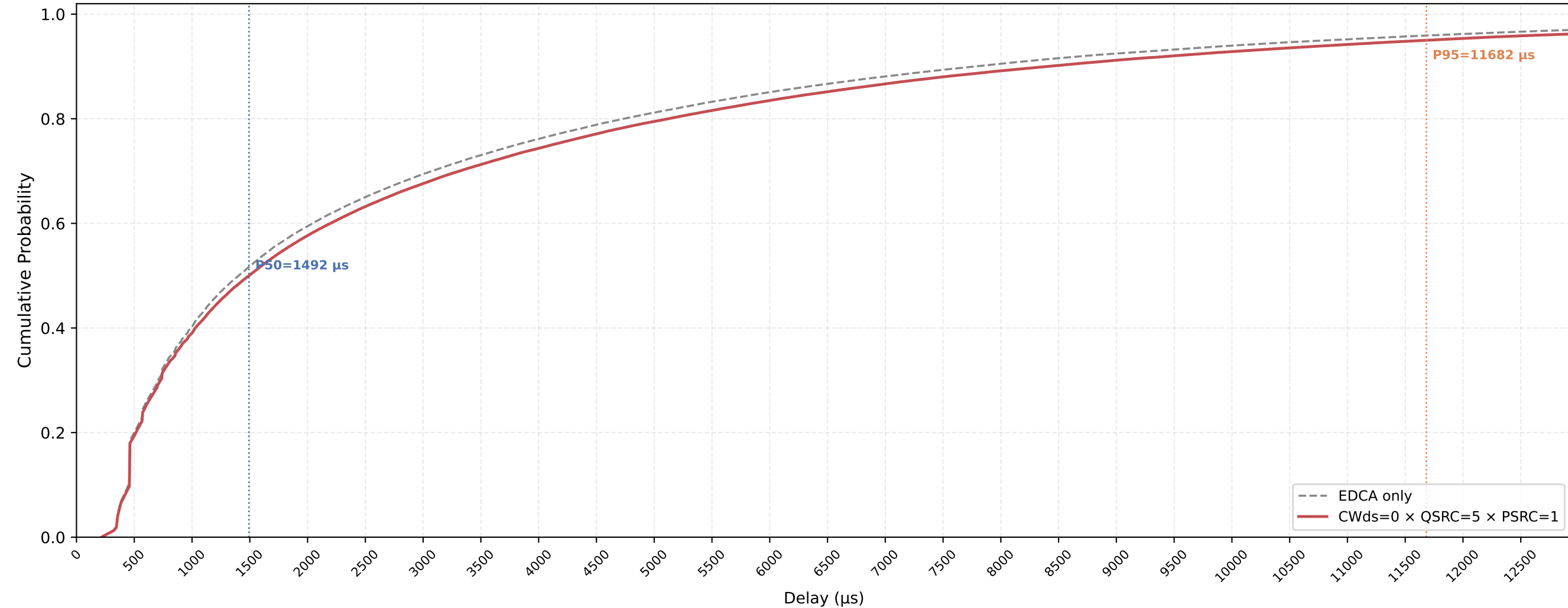
Legacy STA VO Delay CDF — CWds=0 × QSRC=5 × PSRC=1 nSta=30, nPedca=5, 1Mbps, avg of 10 runs
