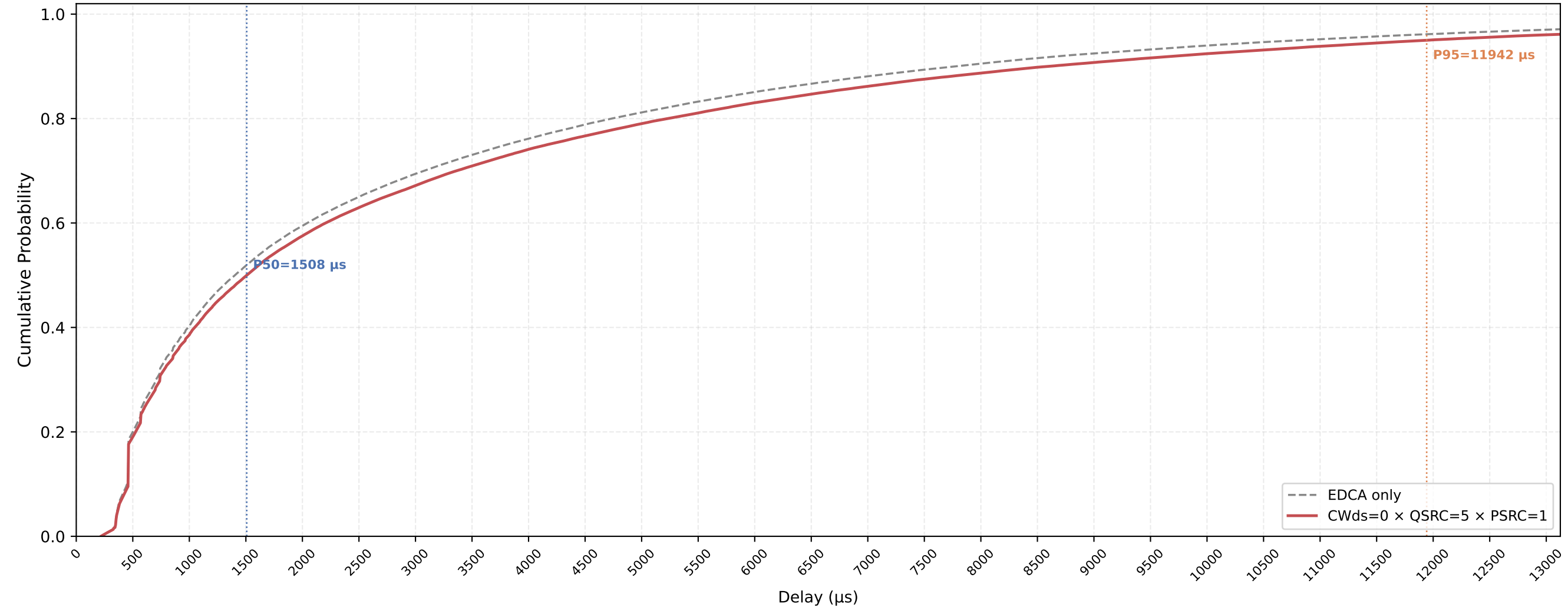
P-EDCA STA VO Delay CDF — CWds=0 × QSRC=5 × PSRC=1 nSta=30, nPedca=15, 1Mbps, avg of 10 runs
