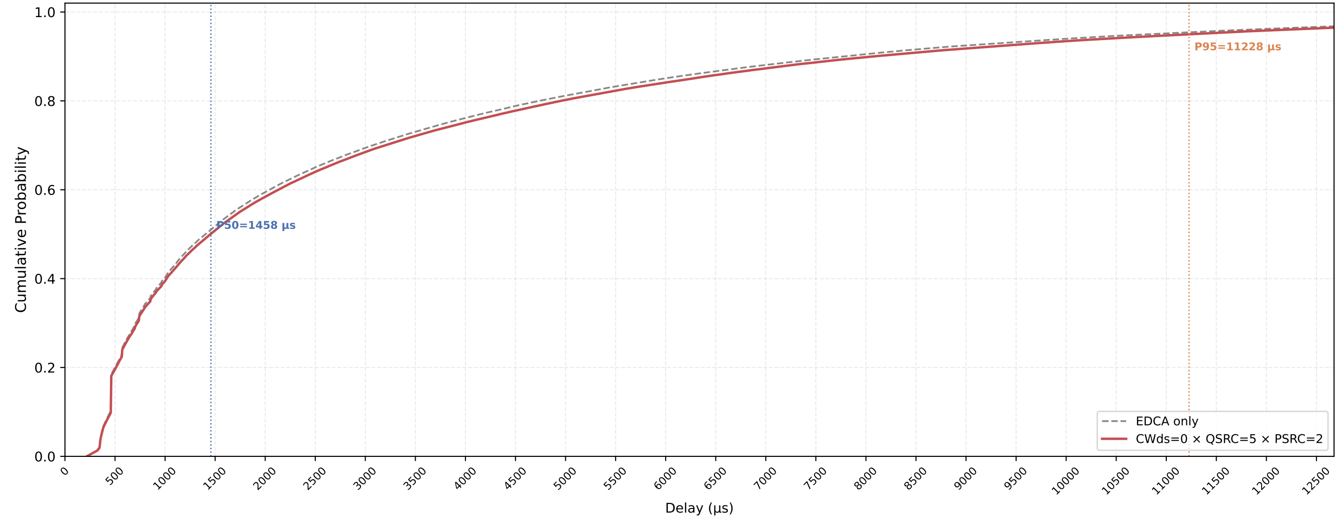
Legacy STA VO Delay CDF — CWds=0 × QSRC=5 × PSRC=2 nSta=30, nPedca=5, 1Mbps, avg of 10 runs
