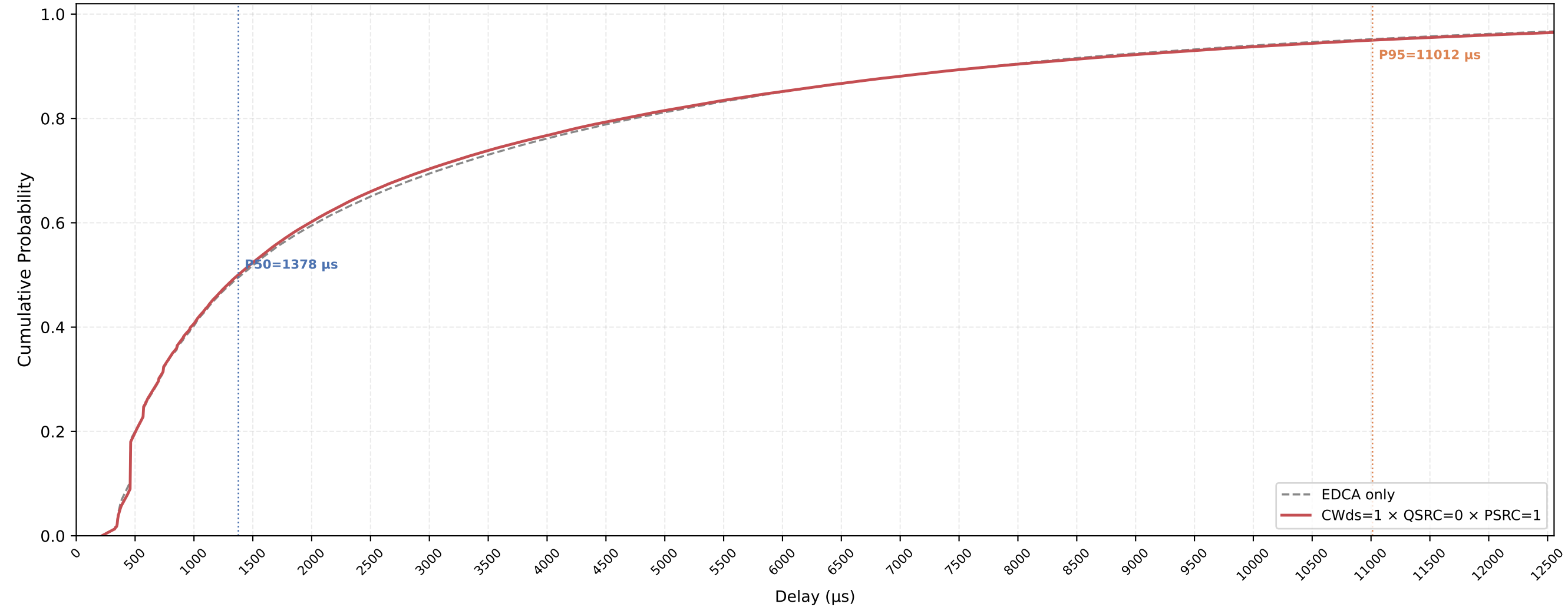
VO (all STAs) Delay CDF — CWds=1 × QSRC=0 × PSRC=1 nSta=30, nPedca=5, 1Mbps, avg of 10 runs
