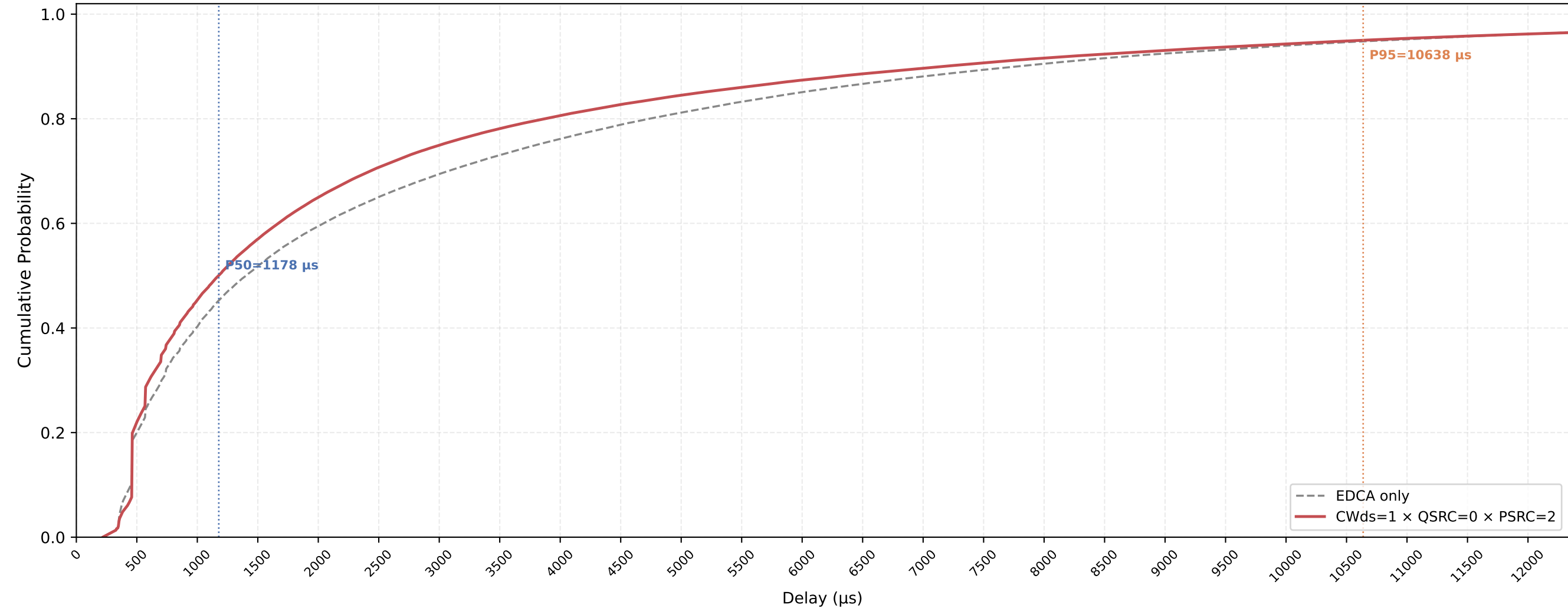
VO (all STAs) Delay CDF — CWds=1 × QSRC=0 × PSRC=2 nSta=30, nPedca=15, 1Mbps, avg of 10 runs
