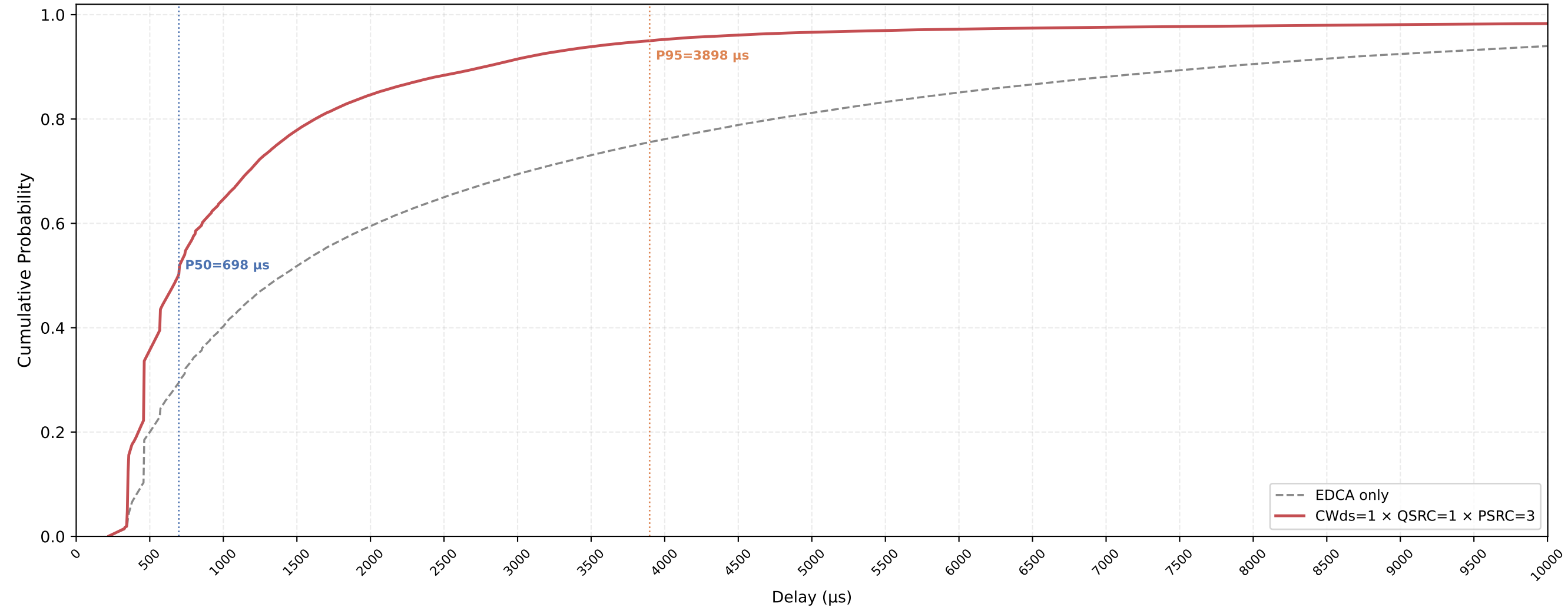
VO (all STAs) Delay CDF — CWds=1 × QSRC=1 × PSRC=3 nSta=30, nPedca=30, 1Mbps, avg of 10 runs
