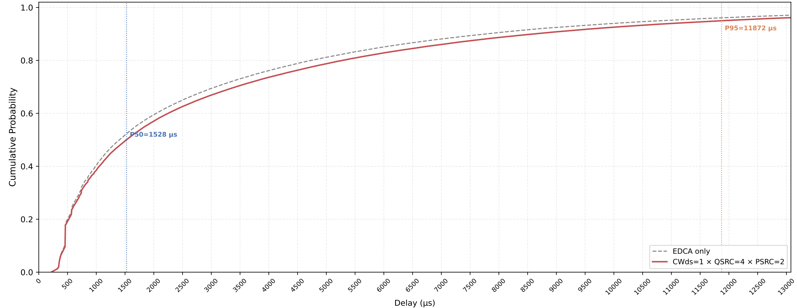
Legacy STA VO Delay CDF — CWds=1 × QSRC=4 × PSRC=2 nSta=30, nPedca=5, 1Mbps, avg of 10 runs
