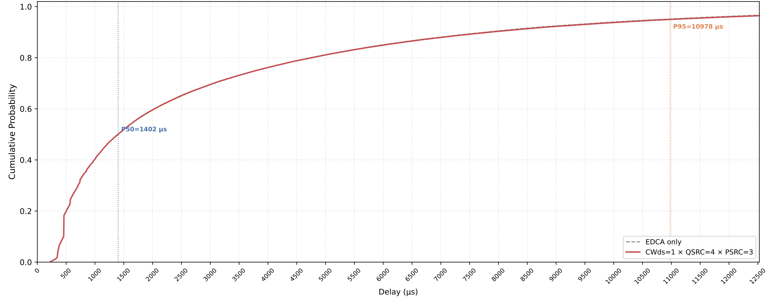
VO (all STAs) Delay CDF — CWds=1 × QSRC=4 × PSRC=3 nSta=30, nPedca=5, 1Mbps, avg of 10 runs
