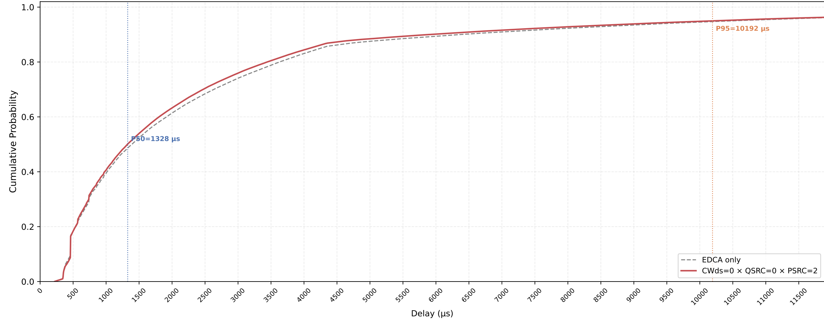
VO (all STAs) Delay CDF — CWds=0 × QSRC=0 × PSRC=2 nSta=30, nPedca=5, 1Mbps, avg of 10 runs
