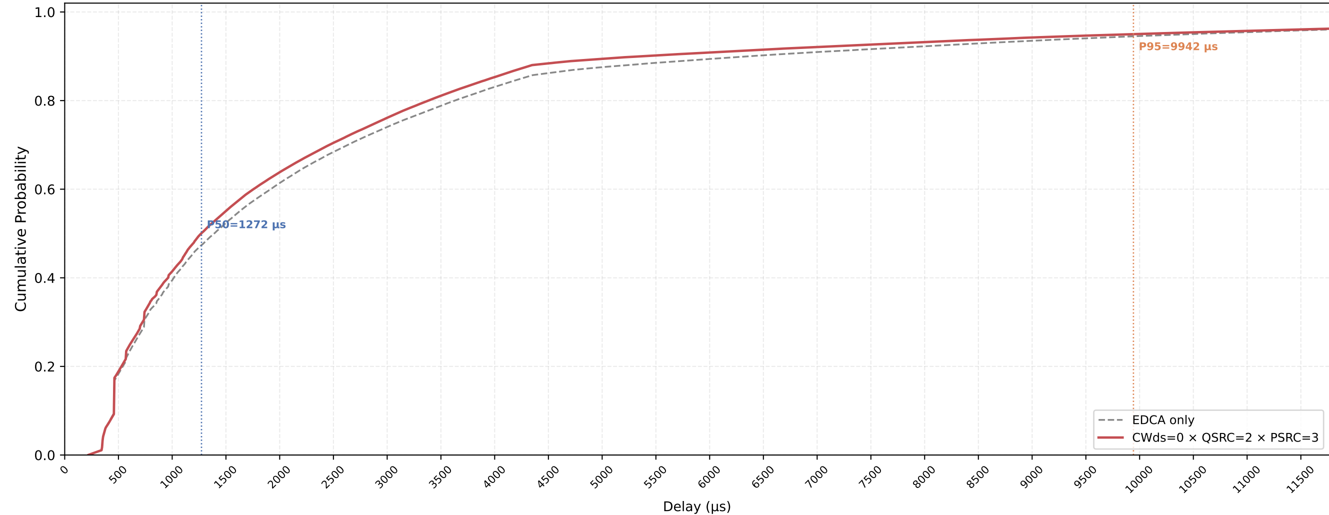
VO (all STAs) Delay CDF — CWds=0 × QSRC=2 × PSRC=3 nSta=30, nPedca=15, 1Mbps, avg of 10 runs
