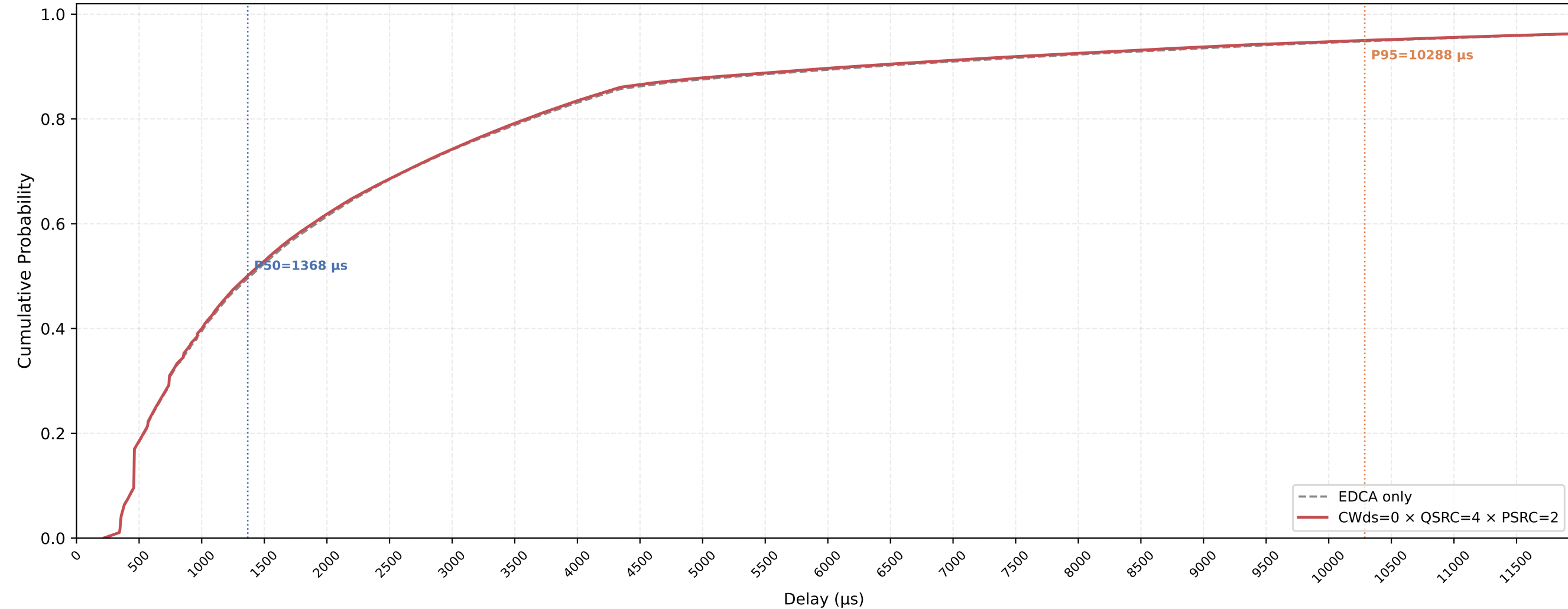
VO (all STAs) Delay CDF — CWds=0 × QSRC=4 × PSRC=2 nSta=30, nPedca=15, 1Mbps, avg of 10 runs
