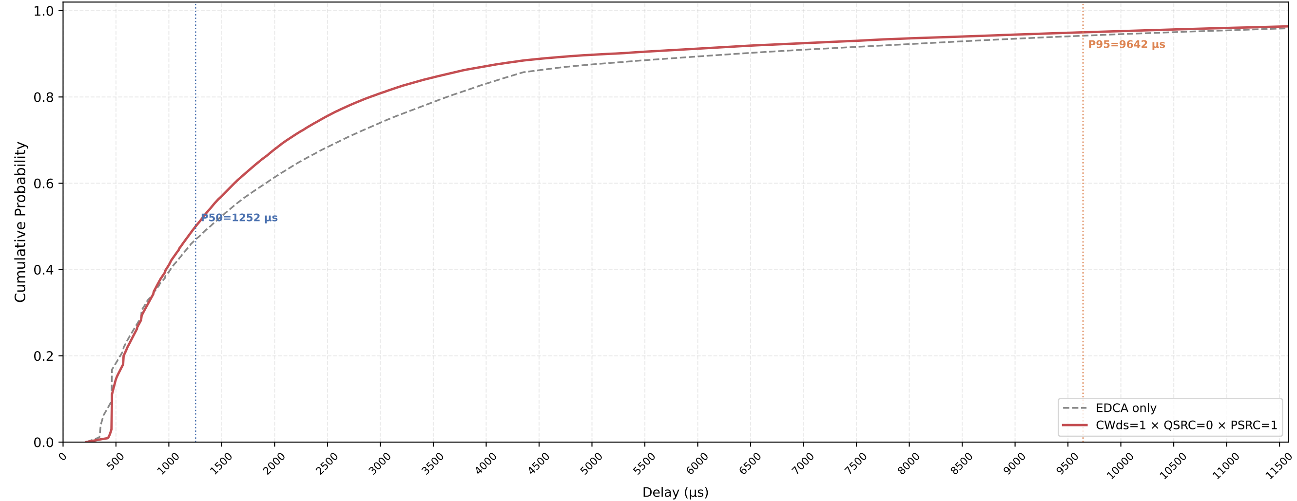
P-EDCA STA VO Delay CDF — CWds=1 × QSRC=0 × PSRC=1 nSta=30, nPedca=15, 1Mbps, avg of 10 runs
