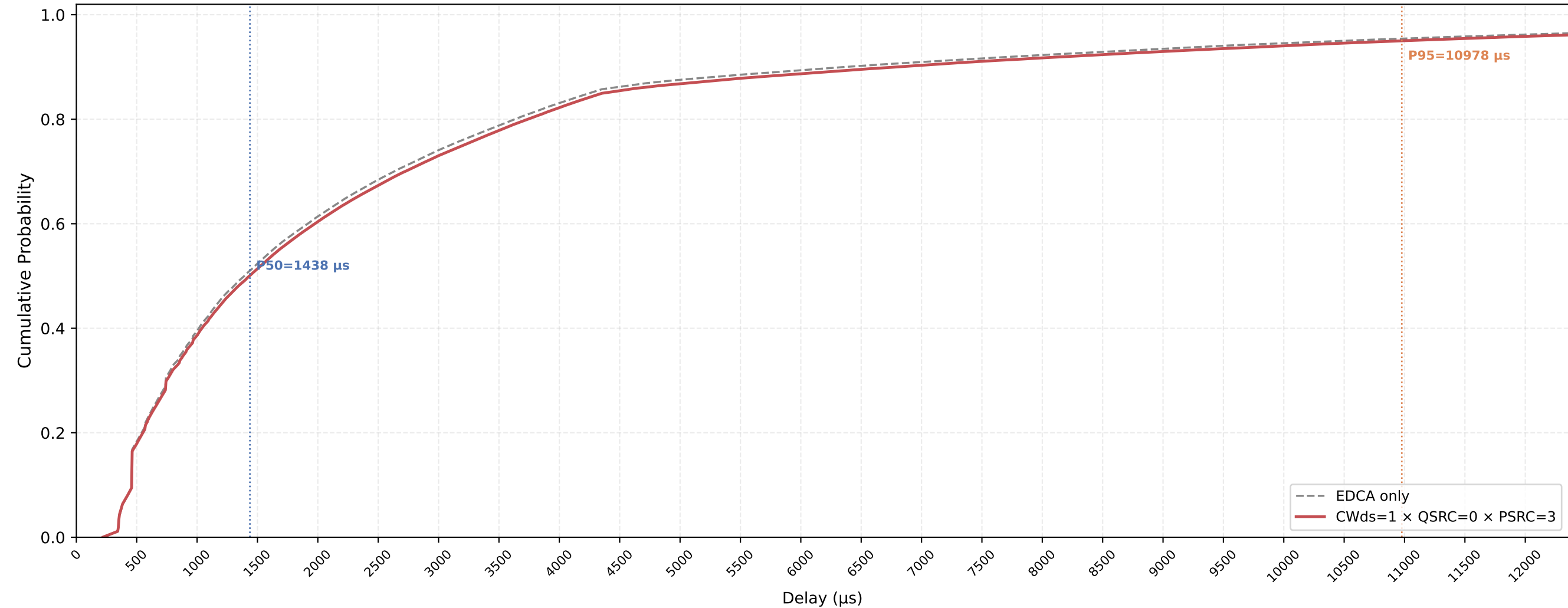
Legacy STA VO Delay CDF — CWds=1 × QSRC=0 × PSRC=3 nSta=30, nPedca=5, 1Mbps, avg of 10 runs
