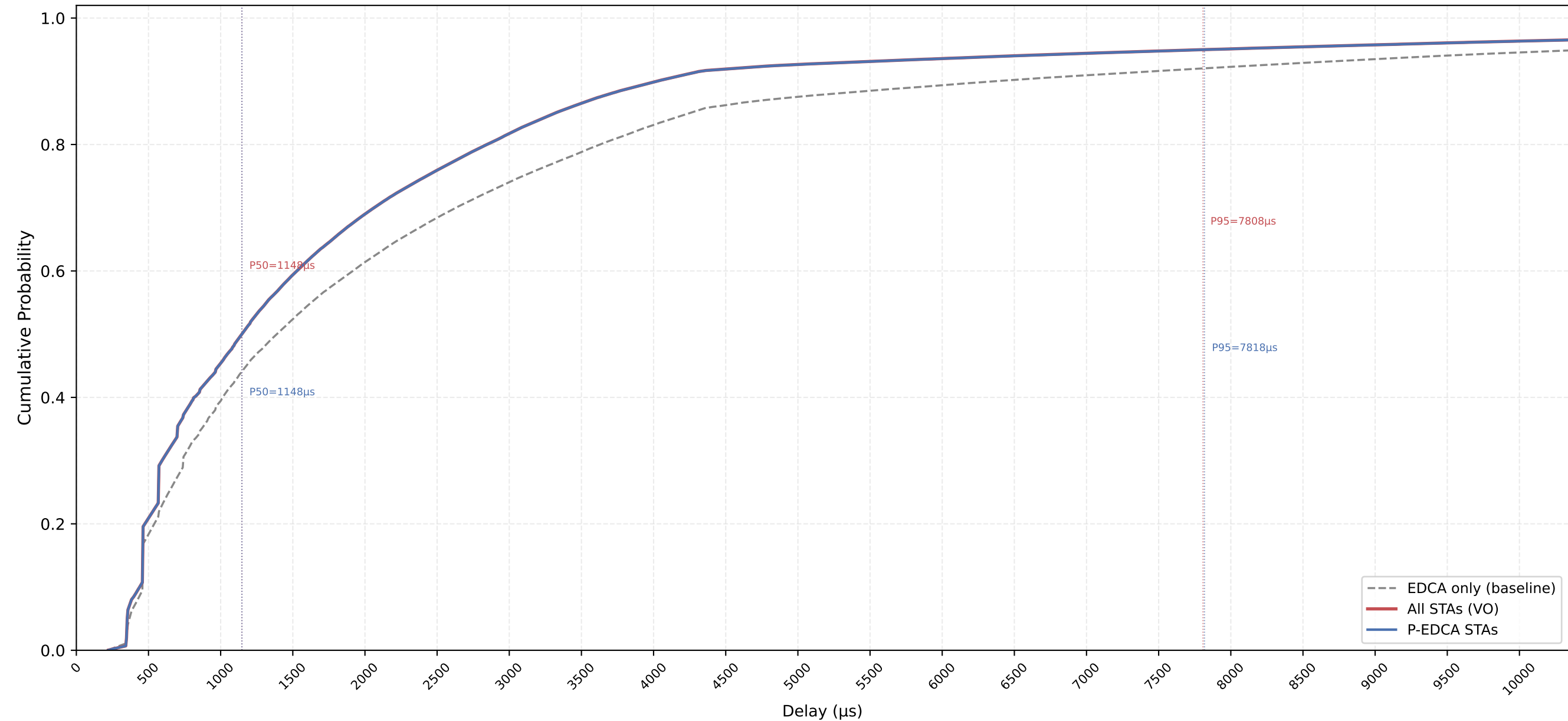
VO Delay CDF — P-EDCA / Legacy / All | CWds=1 × QSRC=1 × PSRC=2 nSta=30, nPedca=30/30, 1Mbps, avg of 10 runs
