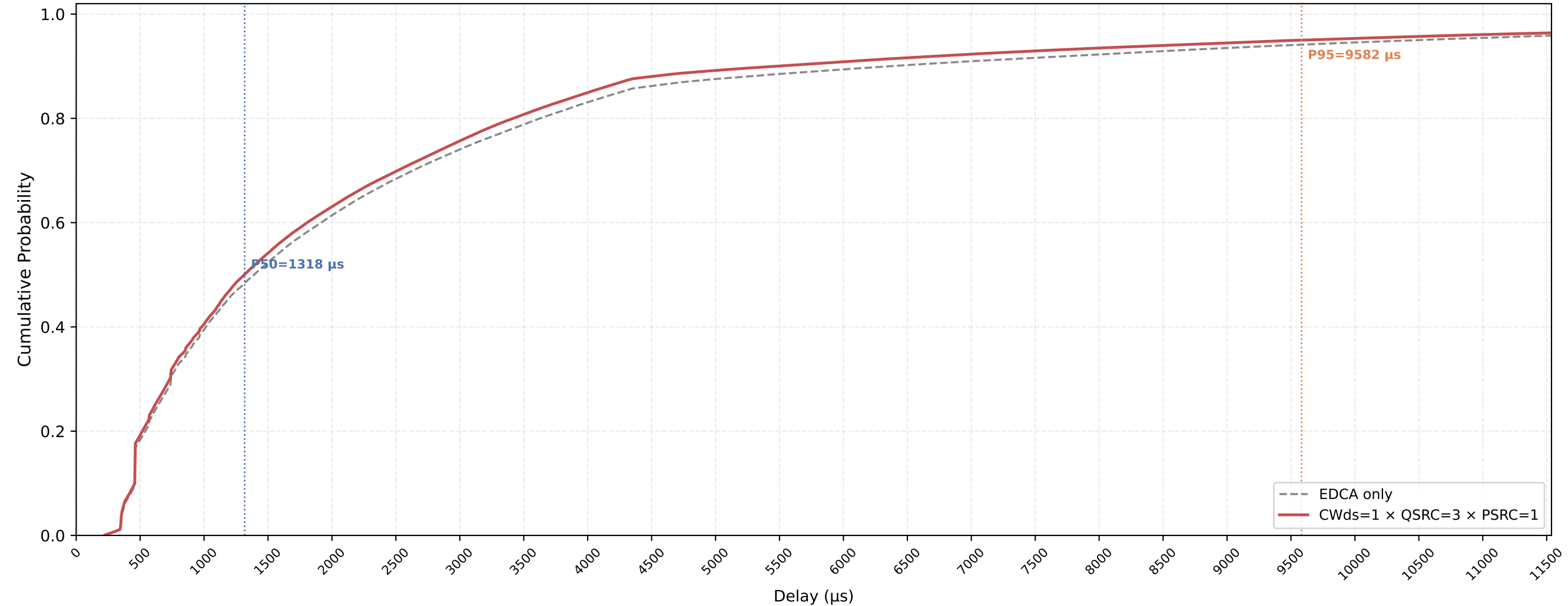
VO (all STAs) Delay CDF — CWds=1 × QSRC=3 × PSRC=1 nSta=30, nPedca=15, 1Mbps, avg of 10 runs
