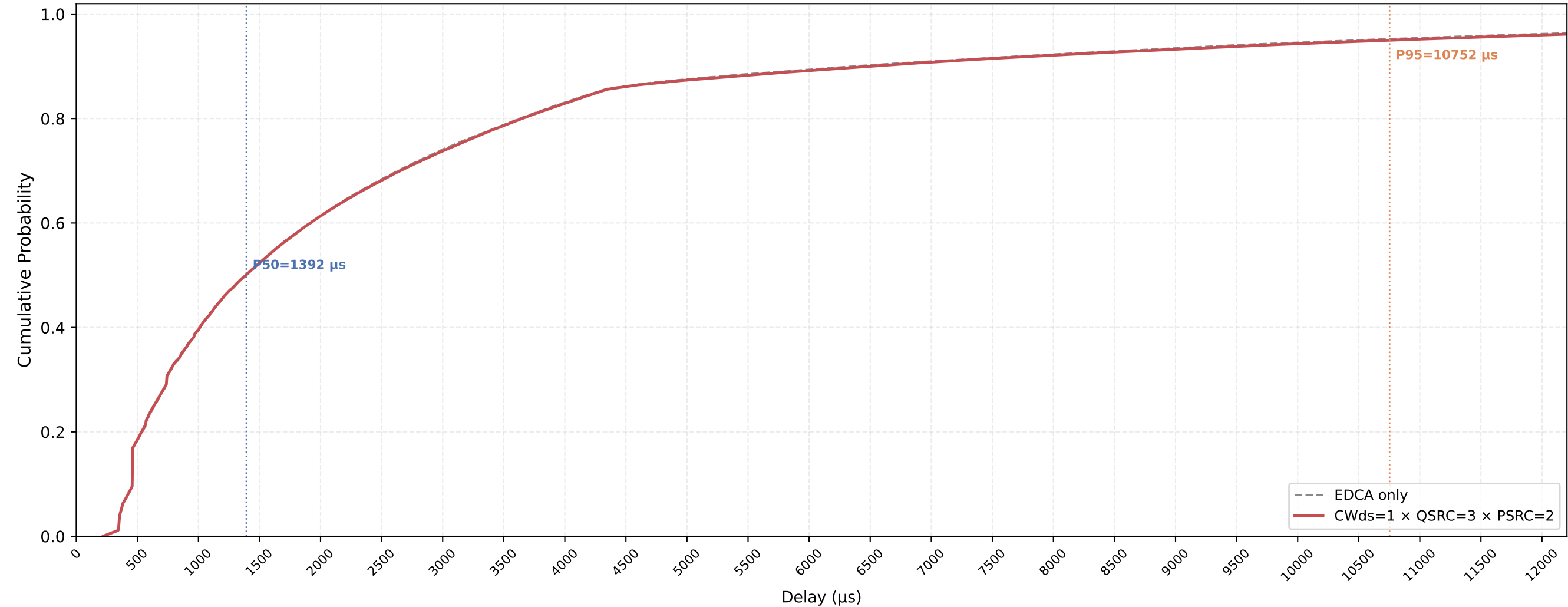
Legacy STA VO Delay CDF — CWds=1 × QSRC=3 × PSRC=2 nSta=30, nPedca=5, 1Mbps, avg of 10 runs
