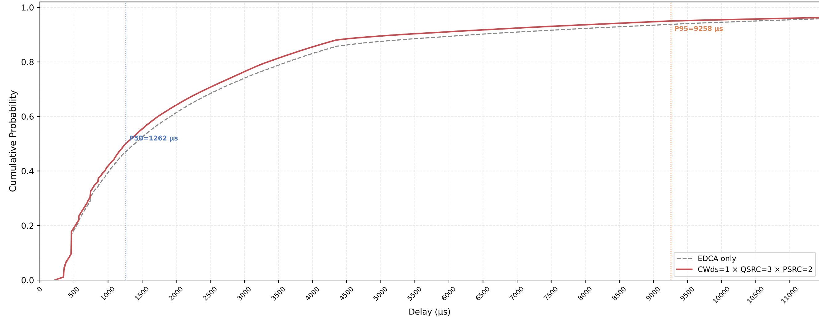
VO (all STAs) Delay CDF — CWds=1 × QSRC=3 × PSRC=2 nSta=30, nPedca=30, 1Mbps, avg of 10 runs
