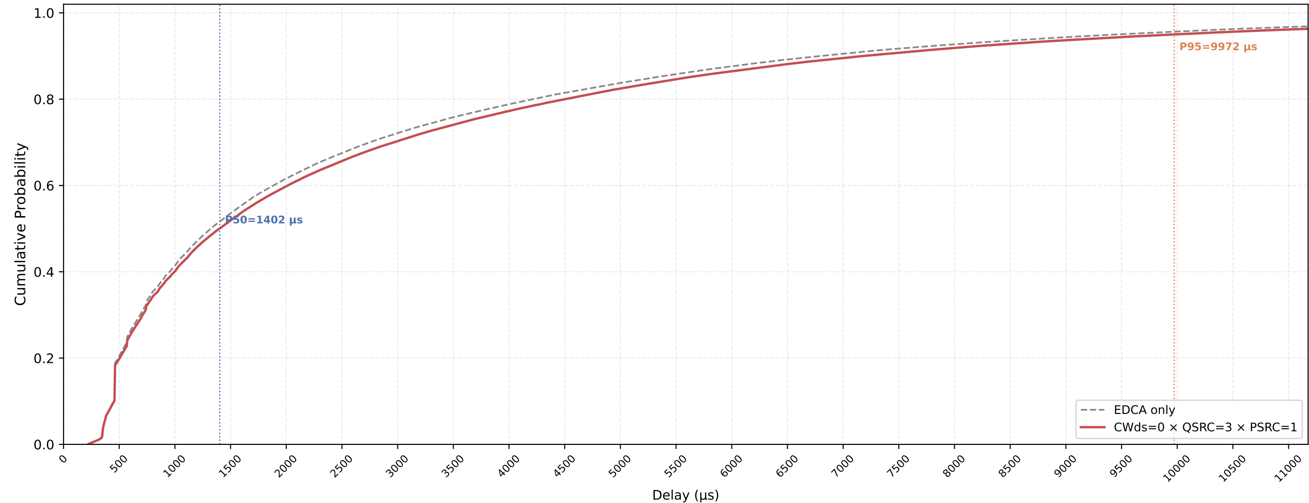
VO (all STAs) Delay CDF — CWds=0 × QSRC=3 × PSRC=1 nSta=30, nPedca=5, 1Mbps, avg of 10 runs
