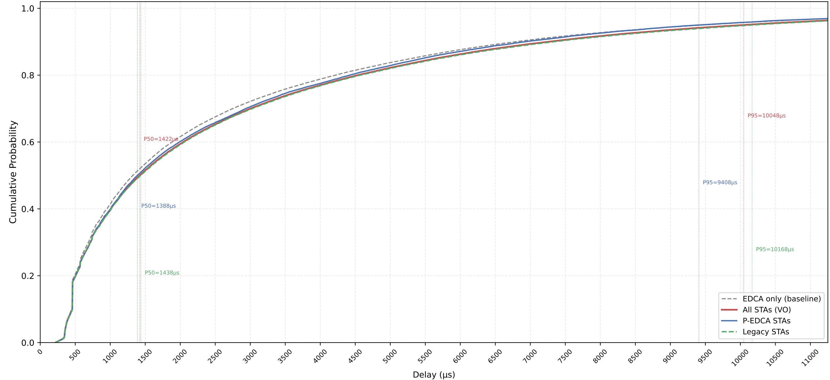
VO Delay CDF — P-EDCA / Legacy / All | CWds=0 × QSRC=4 × PSRC=1 nSta=30, nPedca=5/30, 1Mbps, avg of 10 runs
