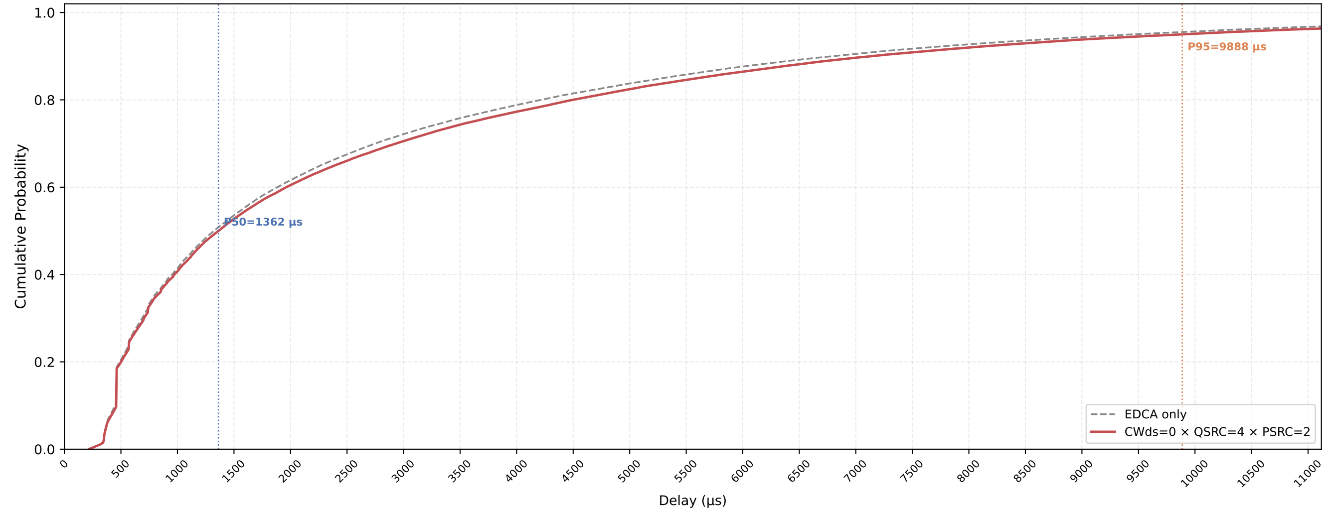
P-EDCA STA VO Delay CDF — CWds=0 × QSRC=4 × PSRC=2 nSta=30, nPedca=15, 1Mbps, avg of 10 runs
