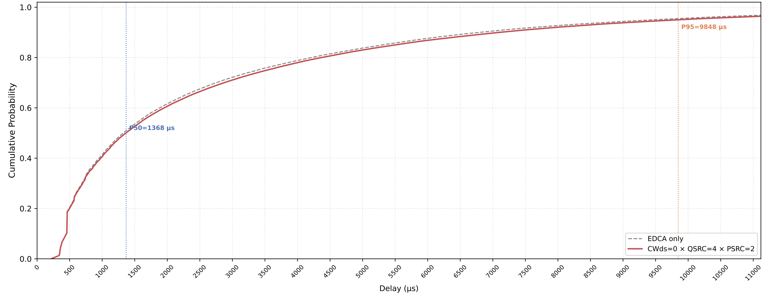
VO (all STAs) Delay CDF — CWds=0 × QSRC=4 × PSRC=2 nSta=30, nPedca=5, 1Mbps, avg of 10 runs
