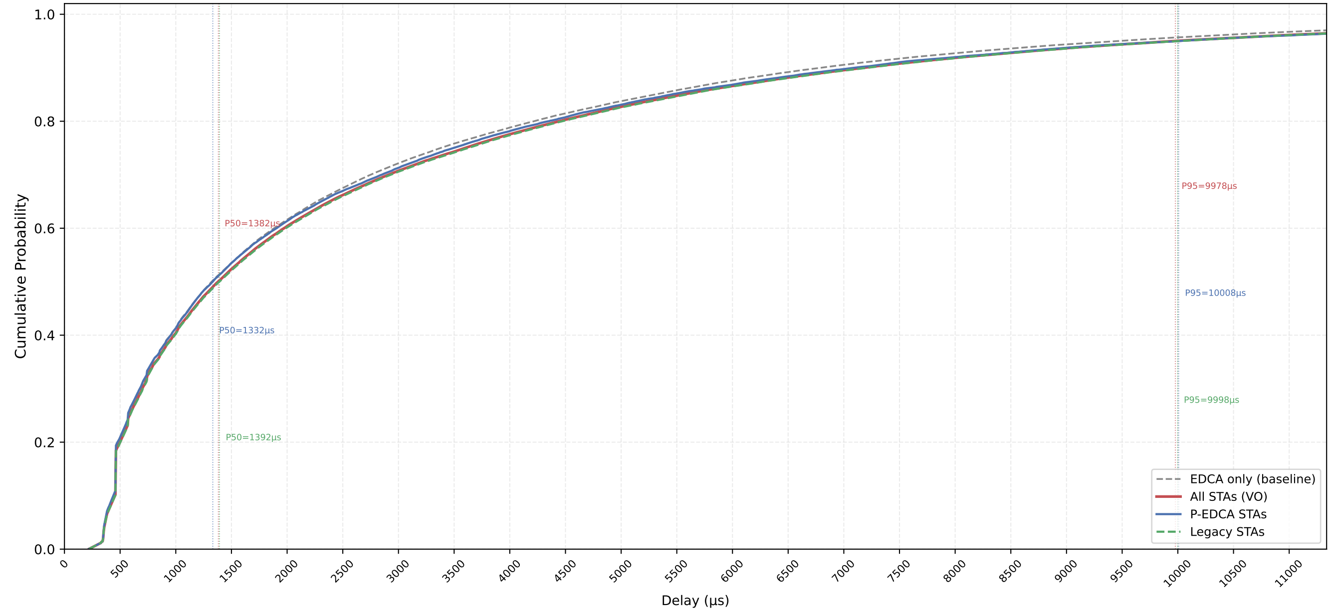
VO Delay CDF — P-EDCA / Legacy / All | CWds=0 × QSRC=5 × PSRC=1 nSta=30, nPedca=5/30, 1Mbps, avg of 10 runs
